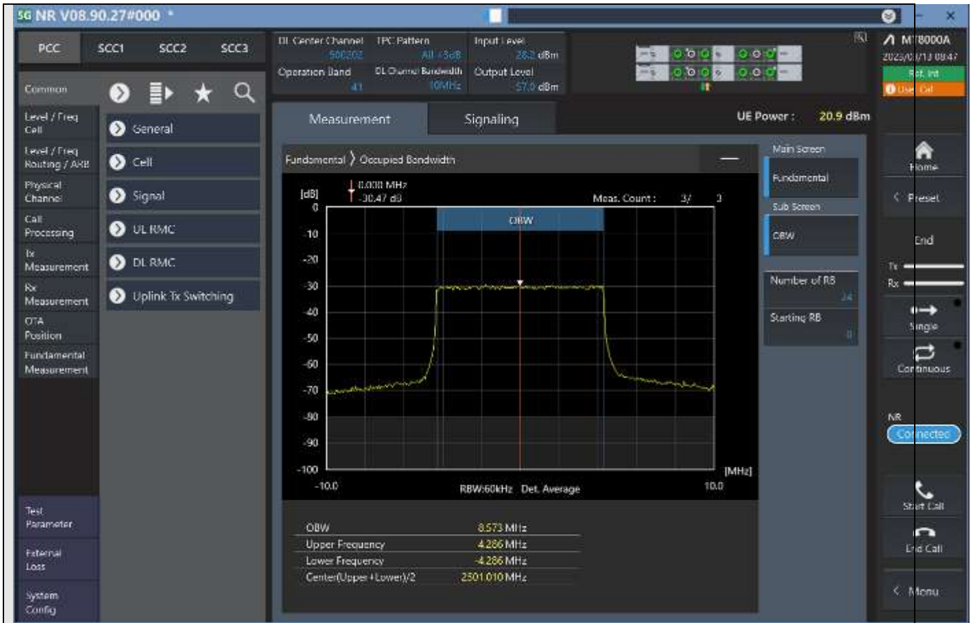
n41_10MHz_30kHz_500202_DFT-s-OFDM 16QAM^Outer_Full
