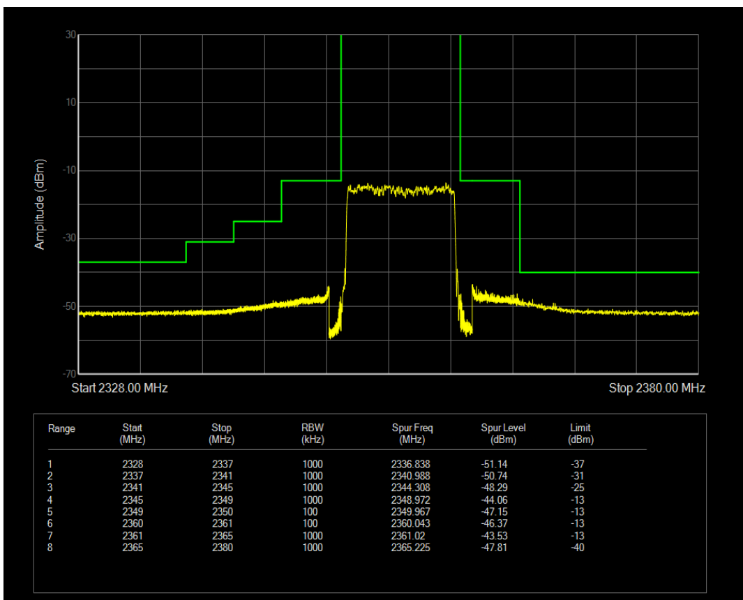
Band40(2350-2360) QAM16 BW=5MHz Channel=39175 RB Size=25 Position=#0
