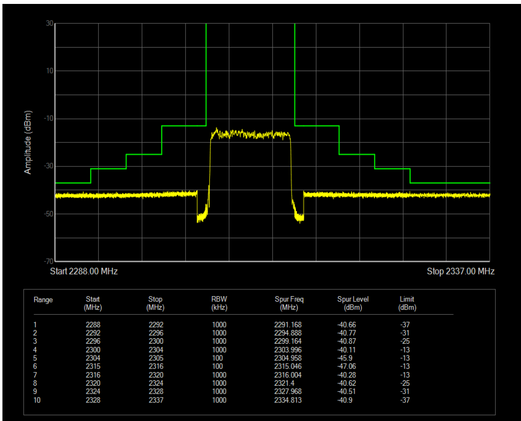
Band40(2305-2315) QAM16 BW=5MHz Channel=38725 RB Size=25 Position=#0
