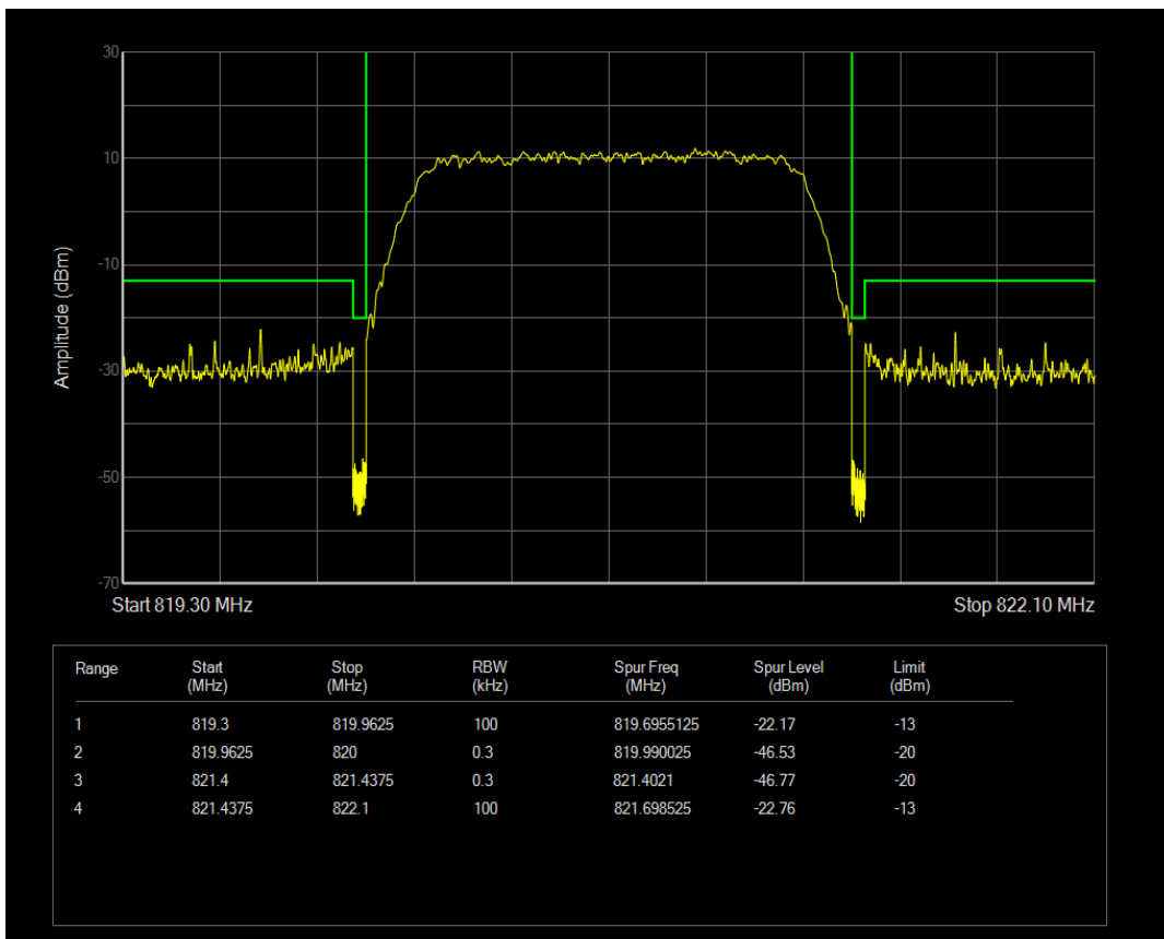
Band26(820-824) QAM16 BW=1.4MHz Channel=26757 RB Size=6 Position=#0
