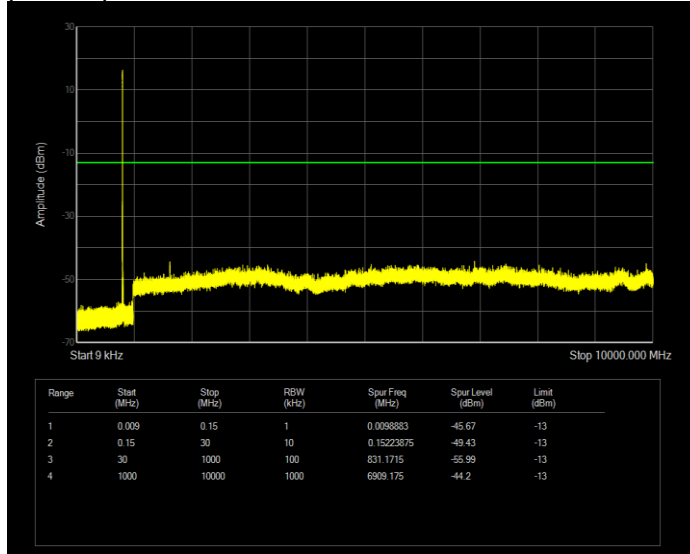
Band26(814-824) QAM16 BW=1.4MHz Channel=26783 RB Size=6 Position=#0
