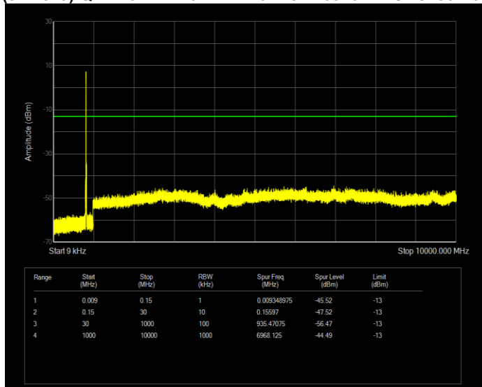
Band26(824-849) QAM16 BW=10MHz Channel=26915 RB Size=50 Position=#0
