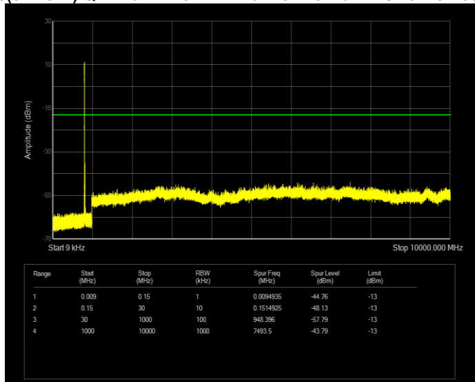
Band26(814-824) QAM16 BW=5MHz Channel=26765 RB Size=25 Position=#0
