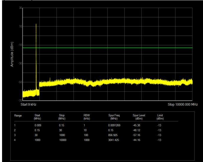
Band26(814-824) QAM16 BW=5MHz Channel=26740 RB Size=25 Position=#0
