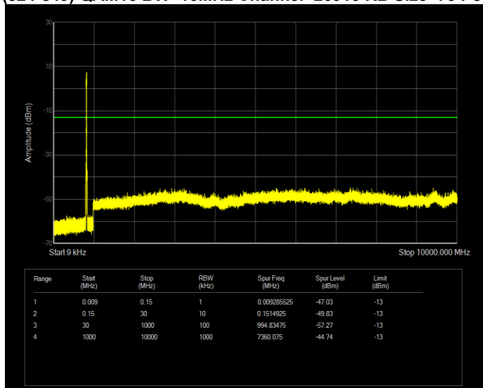
Band26(824-849) QAM16 BW=15MHz Channel=26915 RB Size=75 Position=#0
