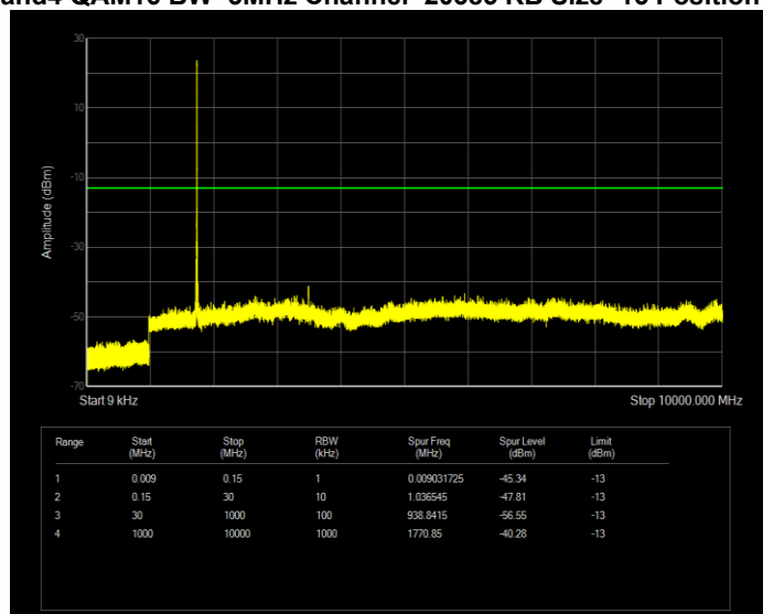
Band4 QAM16 BW=3MHz Channel=20385 RB Size=15 Position=#0
