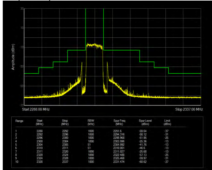
Band4(2305-2315) 16QAM BW=5MHz Channel=38775 RB Size=25 Position=#0
