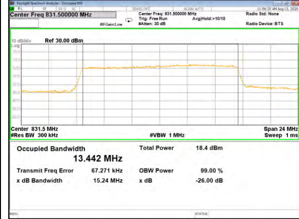
Band26_15M_QPSK_Middle
