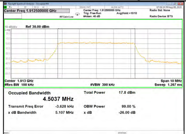
Band25_5M_16QAM_High
