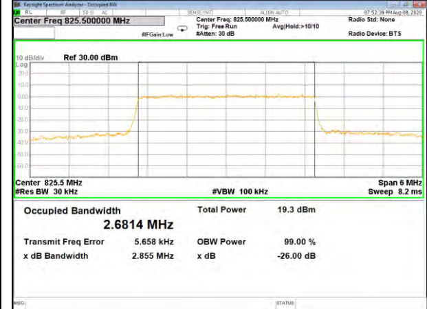
Band26_3M_QPSK_Middle
