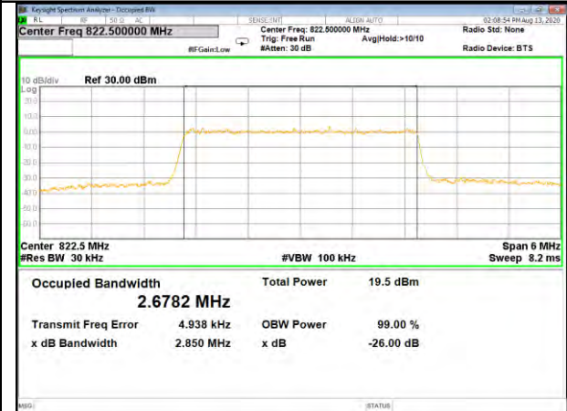
Band26_3M_QPSK_High
