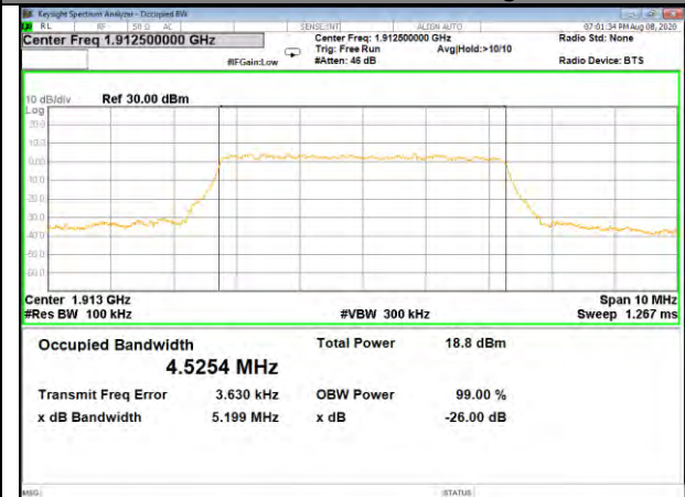
Band25_5M_QPSK_High
