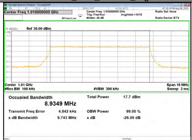
Band25_10M_16QAM_High
