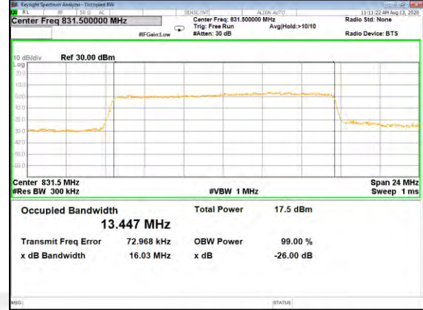
Band26_15M_16QAM_Middle
