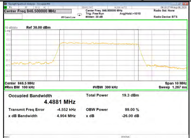
Band26_5M_16QAM_High
