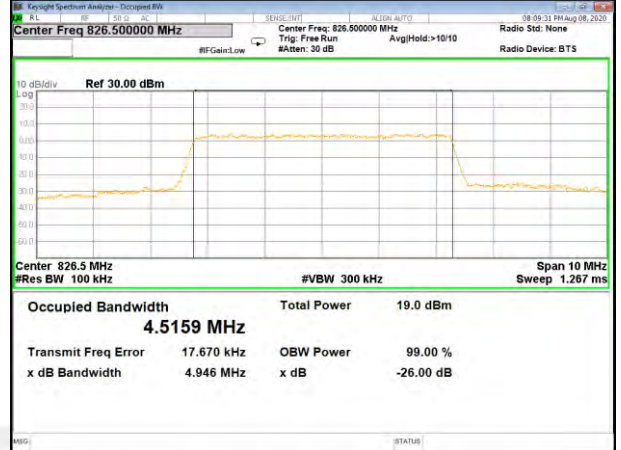
Band26_5M_16QAM_Middle
