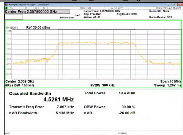
Band40_5M_16QAM_High
