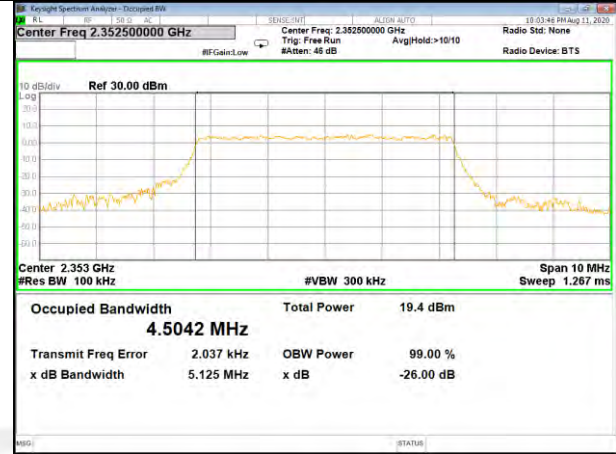
Band40_5M_16QAM_Middle
