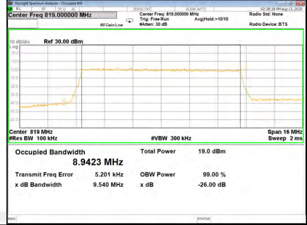
Band26_10M_16QAM_Middle
