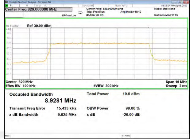
Band26_10M_16QAM_Middle
