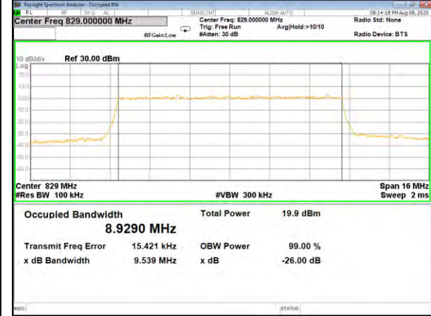
Band26_10M_QPSK_Middle
