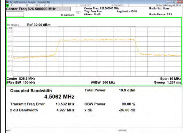
Band26_5M_QPSK_Middle
