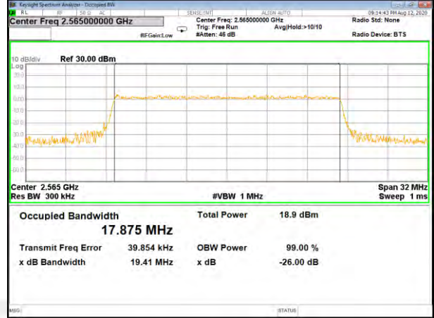
Band41_20M_16QAM_Middle
