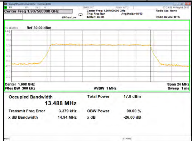
Band25_15M_16QAM_High
