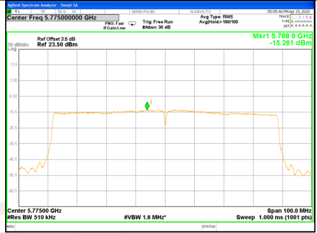
W58_11ac80_Power Density_5775M
