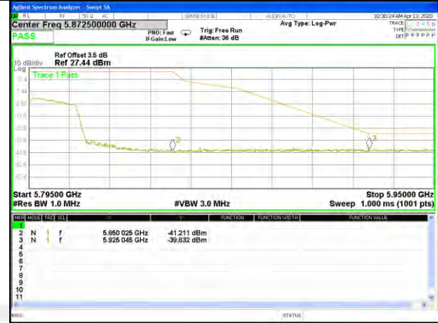
W58_11ac20_Middle_Conducted Spurious
