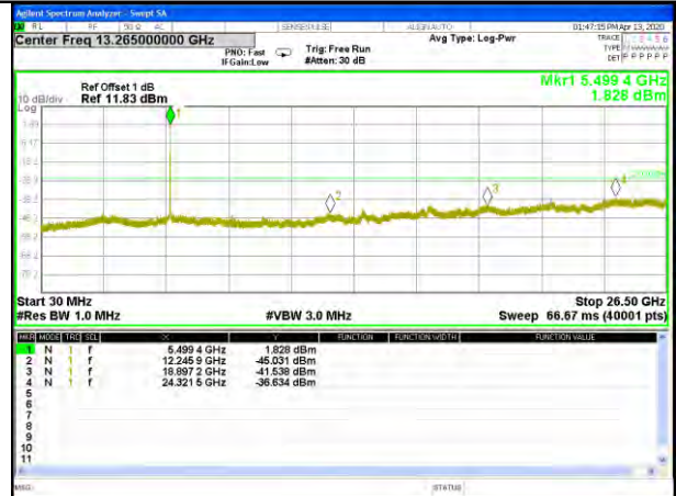
W56_11n20_Lower_Conducted Spurious
