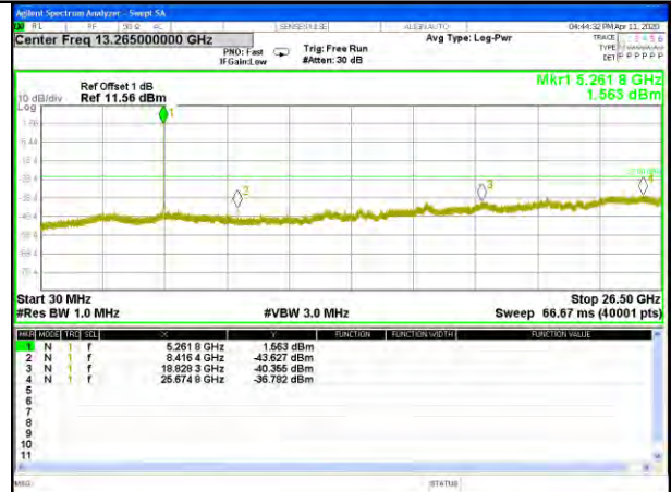
W53_11n20_Lower_Conducted Spurious
