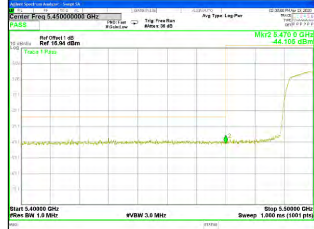
W56_11ac40_Lower_Conducted Spurious
