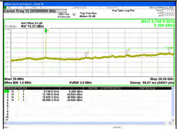
W58_11n20_Lower_Conducted Spurious
