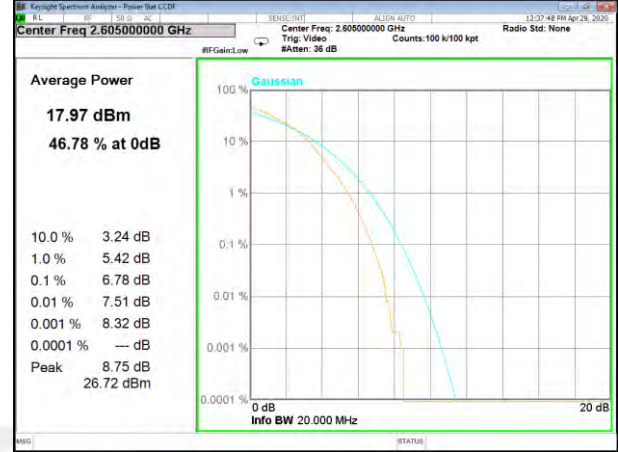
B41_100_QPSK_High_
