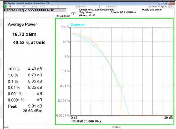
B41_100_QPSK_Middle_
