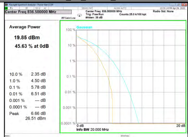
B26_50_QPSK_Middle
