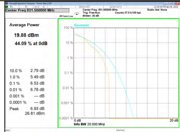
B26_1_QPSK_Middle
