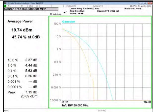
B5_50_QPSK_Middle_
