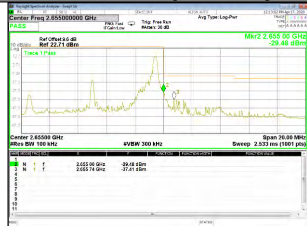
B41_QPSK_10M_High_1-RB_Bedge
