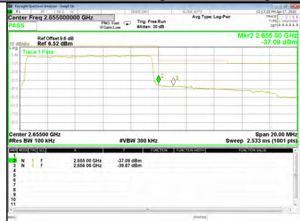
B41_QPSK_10M_High_Full-RB_Bedge
