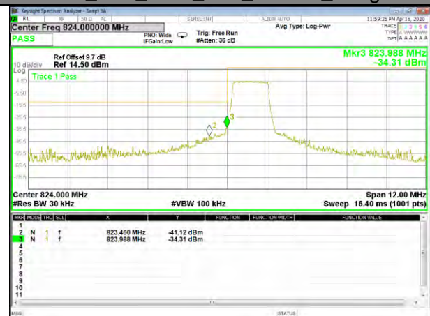
B26_Q16_1.4M_Low_Full-RB_Bedge
