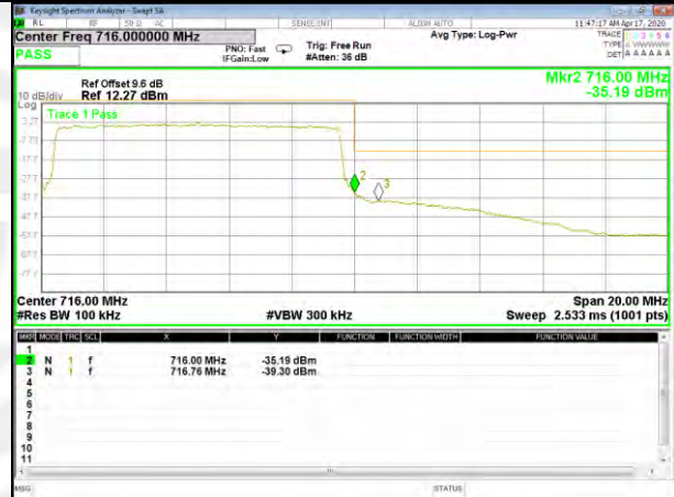
B17_Q16_10M_High_Full-RB_Bedge
