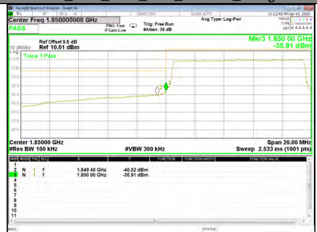
B25_Q16_10M_Low_Full-RB_Bedge
