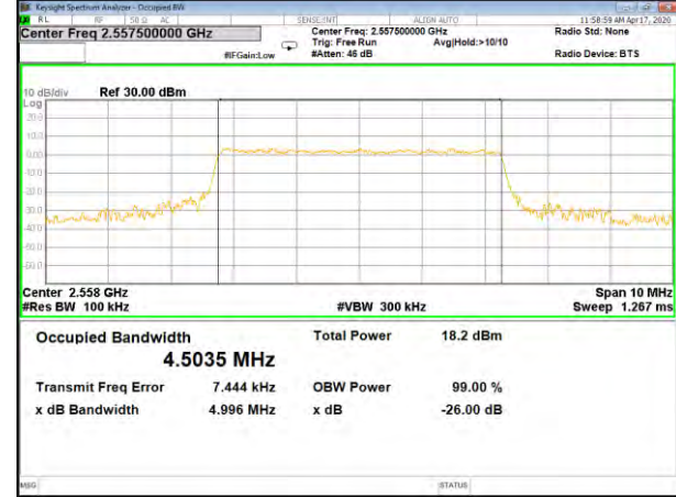
B41_QPSK_5M_Mid_26BW-99%
