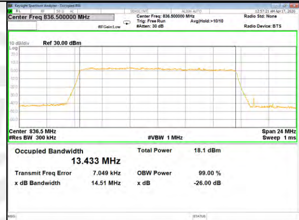
B26_Q16_15M_High_26BW-99%
