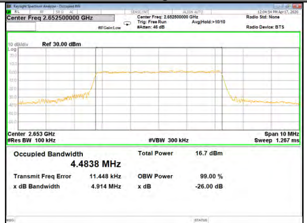
B41_Q16_5M_High_26BW-99%
