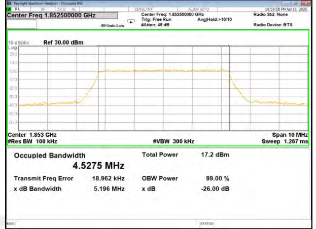
B25_Q16_5M_Mid_26BW-99%
