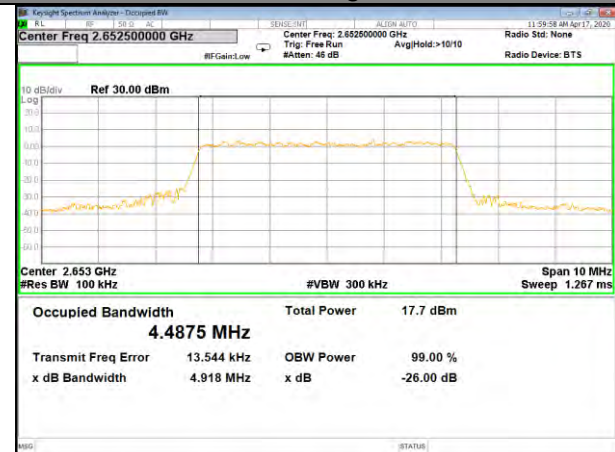
B41_QPSK_5M_High_26BW-99%
