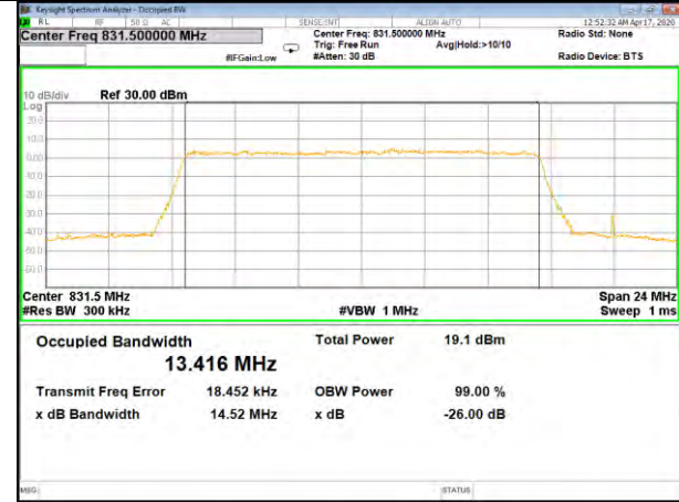
B26_QPSK_15M_Mid_26BW-99%
