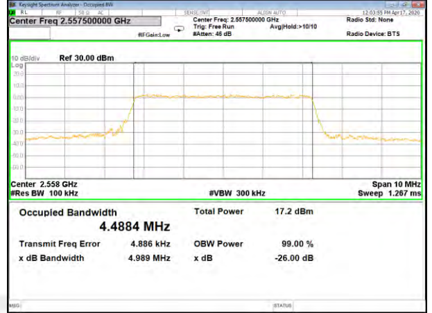
B41_Q16_5M_Mid_26BW-99%
