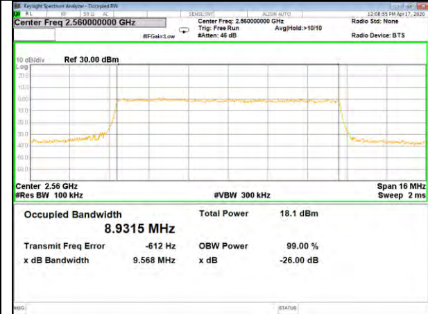
B41_QPSK_10M_Mid_26BW-99%
