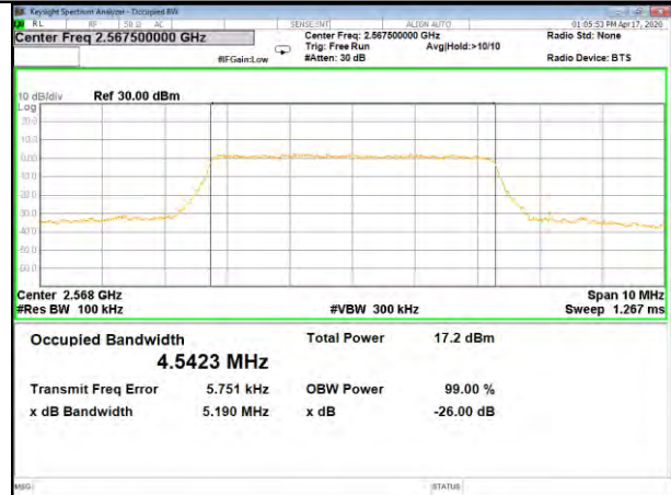
B7_Q16_5M_High_26BW-99%
