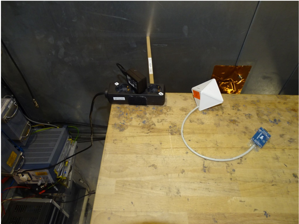
Photo 1: Test setup for conducted measurements
