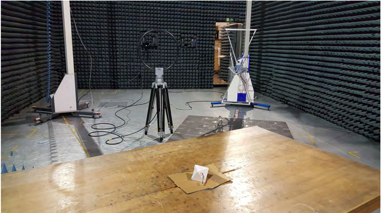
Photo 2: Test setup for radiated measurements (Enclosure, fully-anechoic chamber, 1-18 GHz intentional radiator §15 / 30 MHz – 10/20 GHz §22/24/27)
