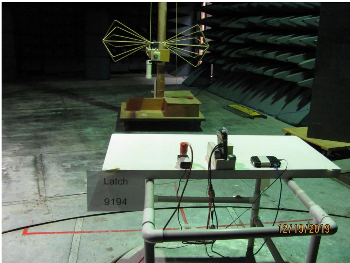
Biconical Antenna
