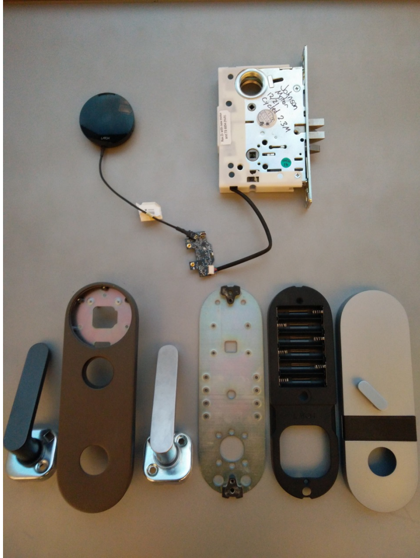
Figure 9 Enclosure Assemblies
