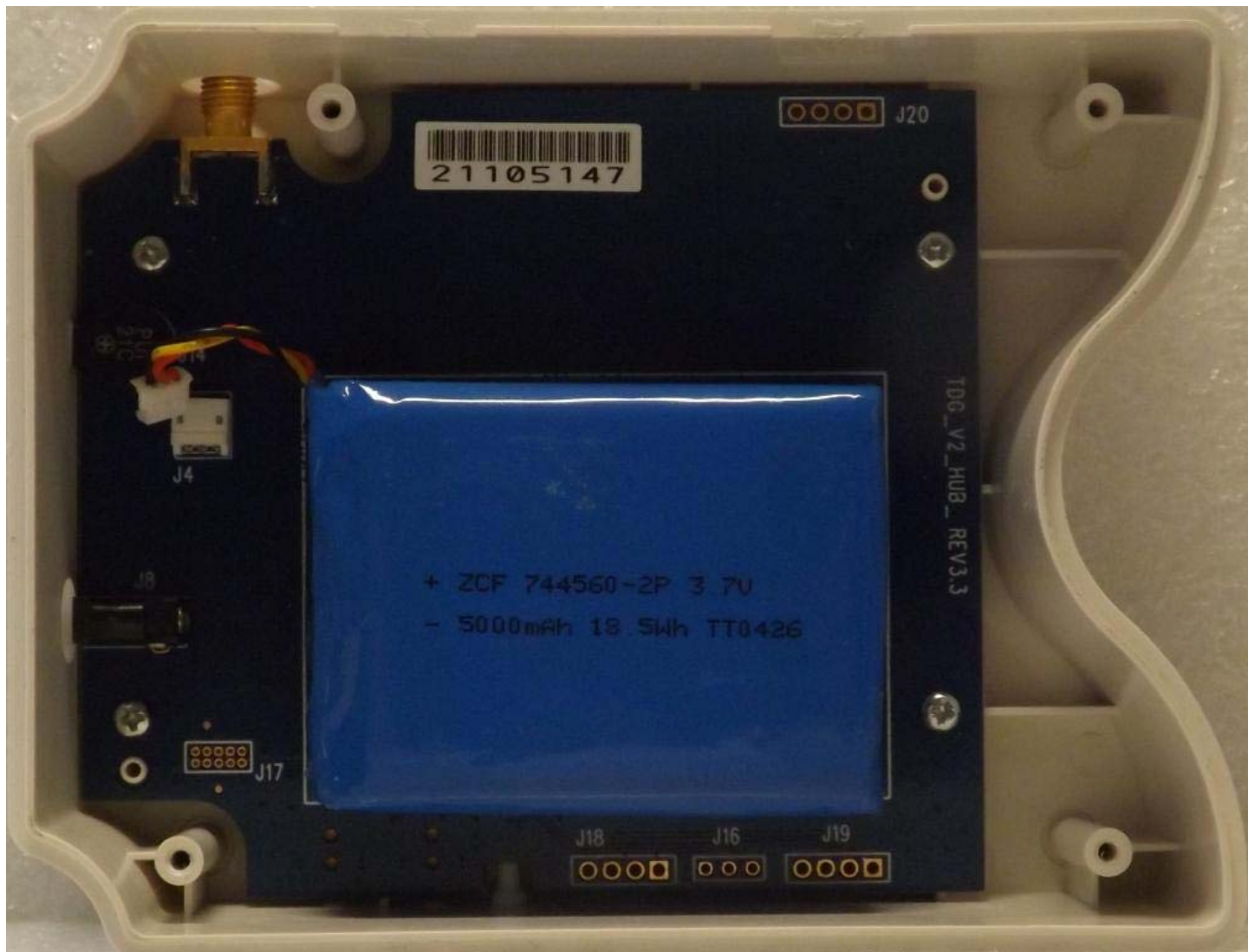
Figure E9.1 – DUT Cover Removed
