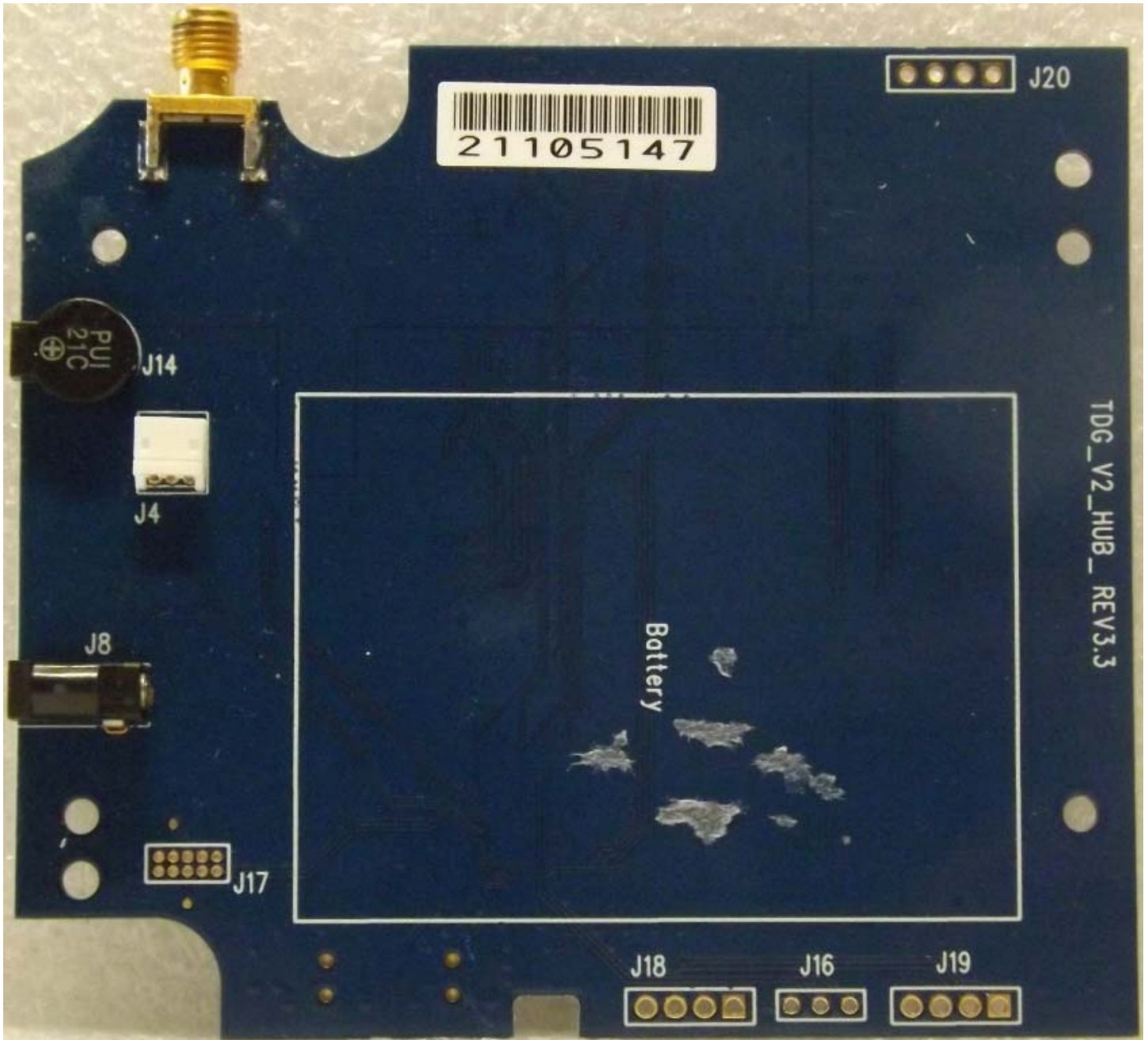
Figure E9.2 – Main PCB, Back Side, Battery Removed
