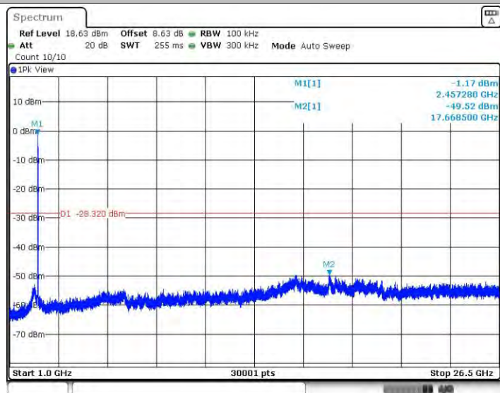
11AX20SISO_Ant1_2462_1000~26500
