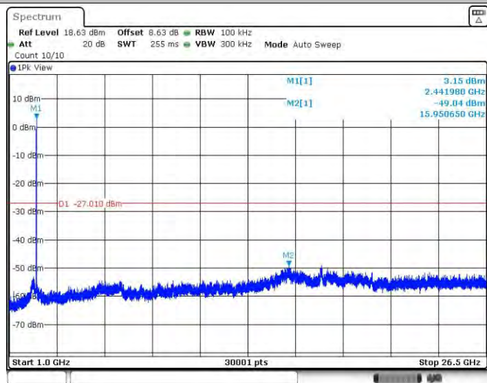
11G_Ant1_2437_1000~26500
