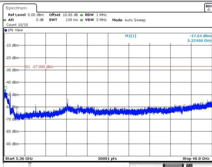
11AX20SISO_Ant1_5320_5360~40000
