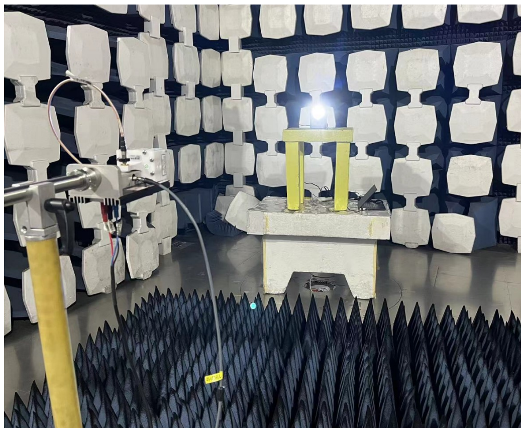
Description: Test Setup
