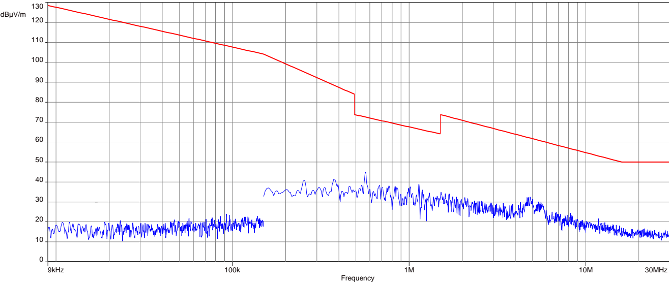
Plot 7: EUT2, 15.209, TX Magnetic
