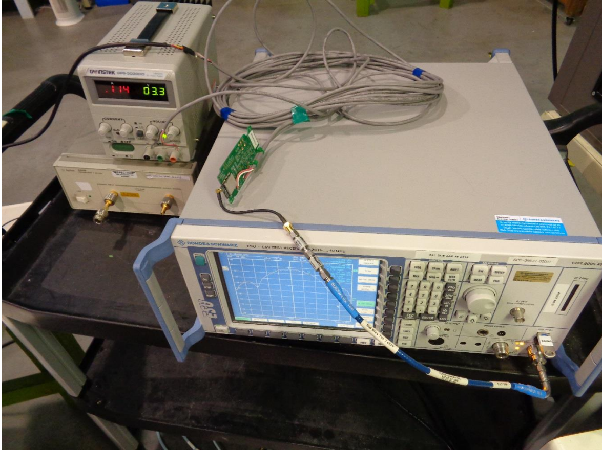
Figure 6 – Conducted Emissions Setup – Photo 5
