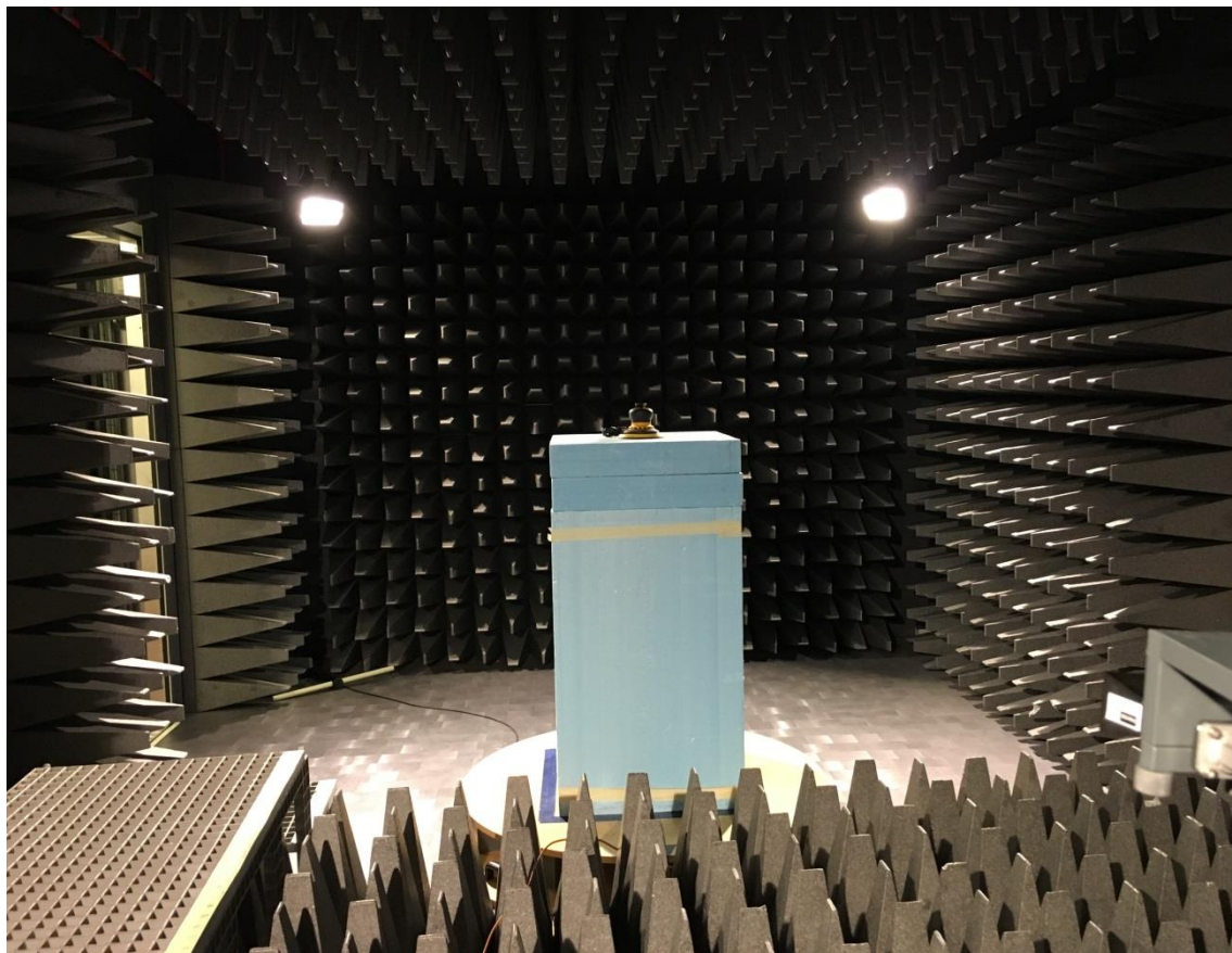
Test set up radiated emission 18 GHz – 26.5 GHz
