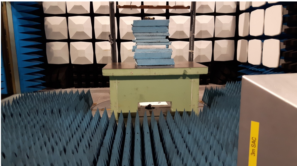
Test set up radiated emission 1GHz – 26.5 GHz
