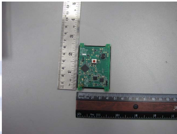
Picture 10: PCBA 1
