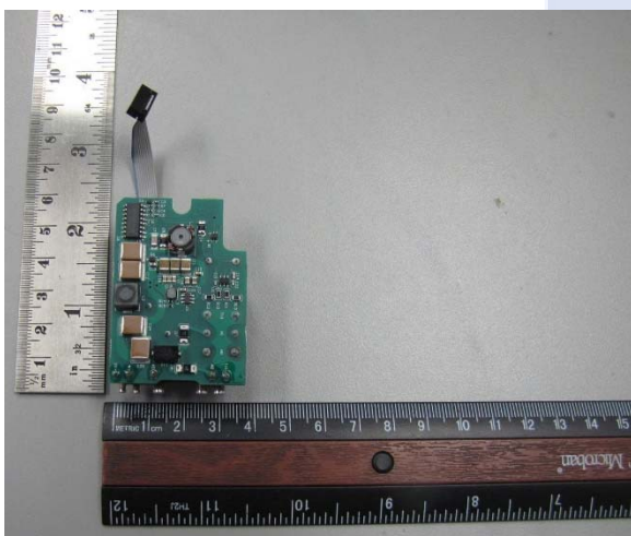
Picture 13: PCBA2 – Bottom View
