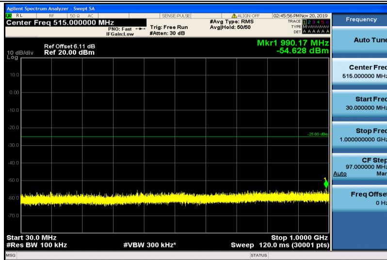
Band41-5MHz-16QAM-41565-1RB#0-30~1000MHz
