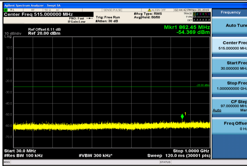
Band41-5MHz-16QAM-40620-1RB#0-30~1000MHz
