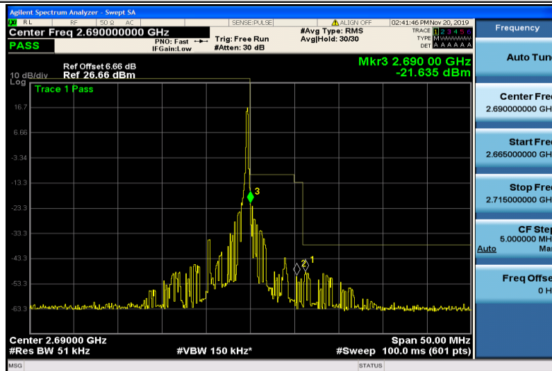
Band41-5MHz-QPSK-41565-1RB#24
