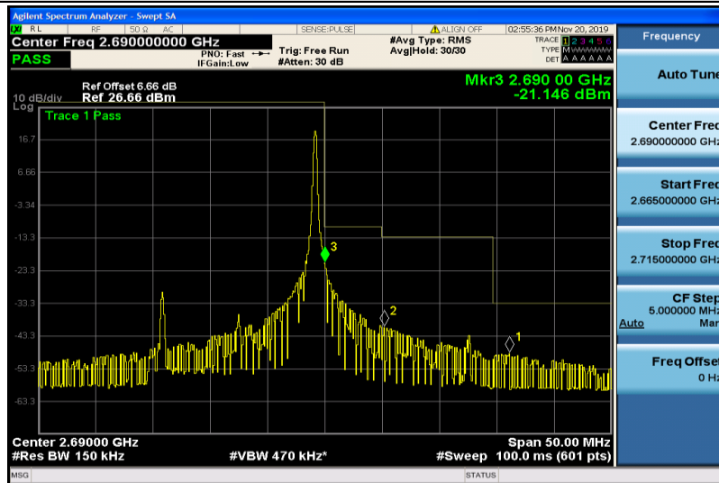
Band41-15MHz-16QAM-41515-1RB#74
