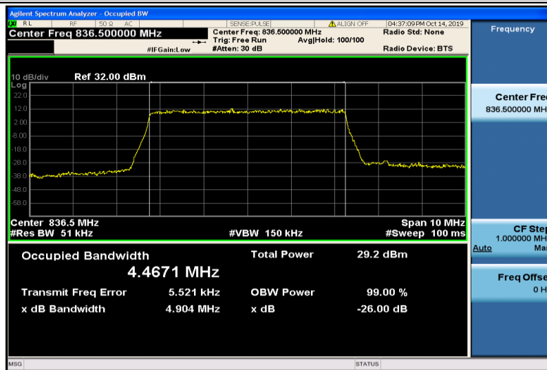
Band5-5MHz-QPSK-20525-25RB#0-4.4671
