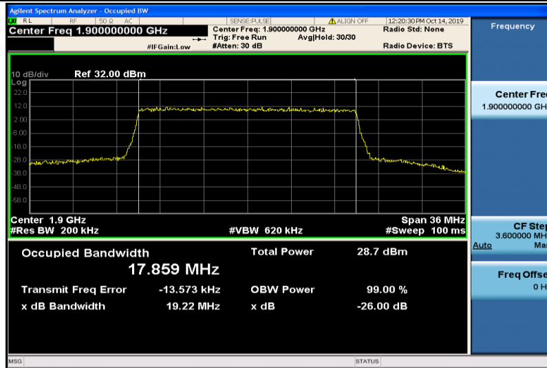
Band2-20MHz-16QAM-19100-100RB#0-17.859
