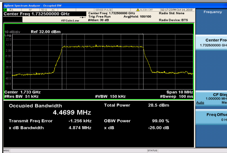
Band4-5MHz-16QAM-20175-25RB#0-4.4699
