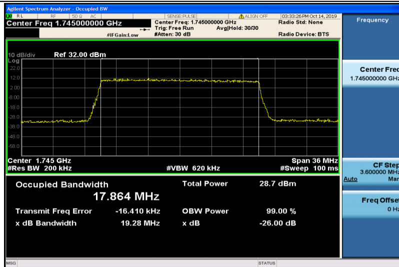
Band4-20MHz-16QAM-20300-100RB#0-17.864
