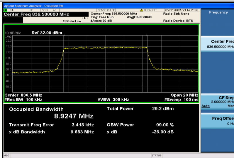
Band5-10MHz-QPSK-20525-50RB#0-8.9247
