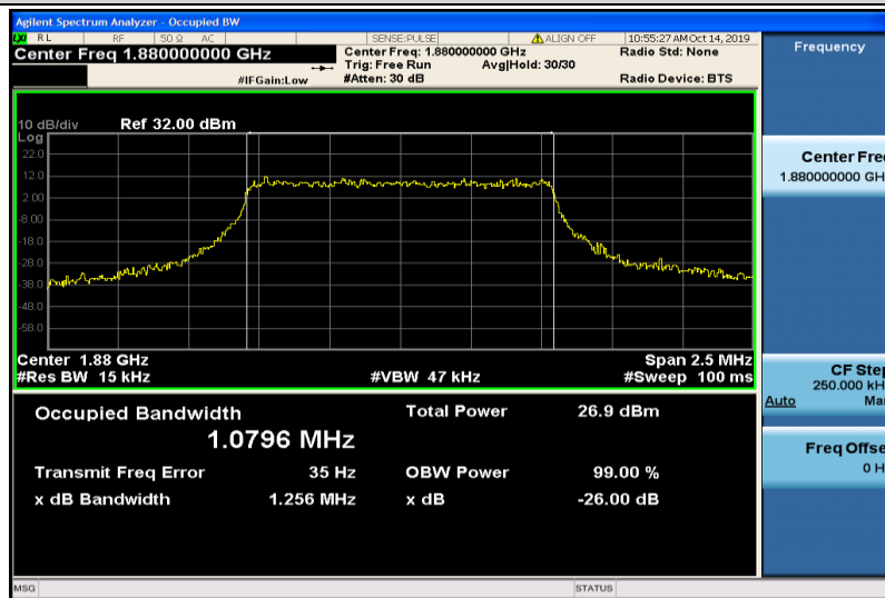
Band2-1.4MHz-16QAM-18900-6RB#0-1.0796
