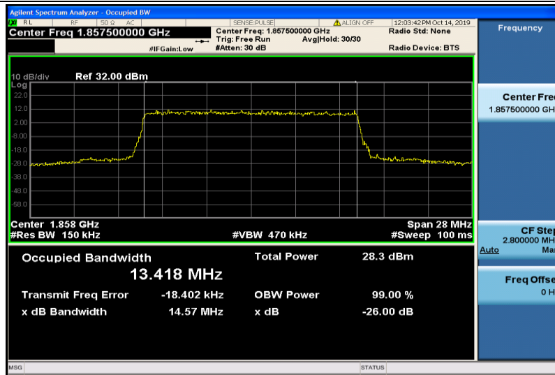
Band2-15MHz-16QAM-18675-75RB#0-13.418
