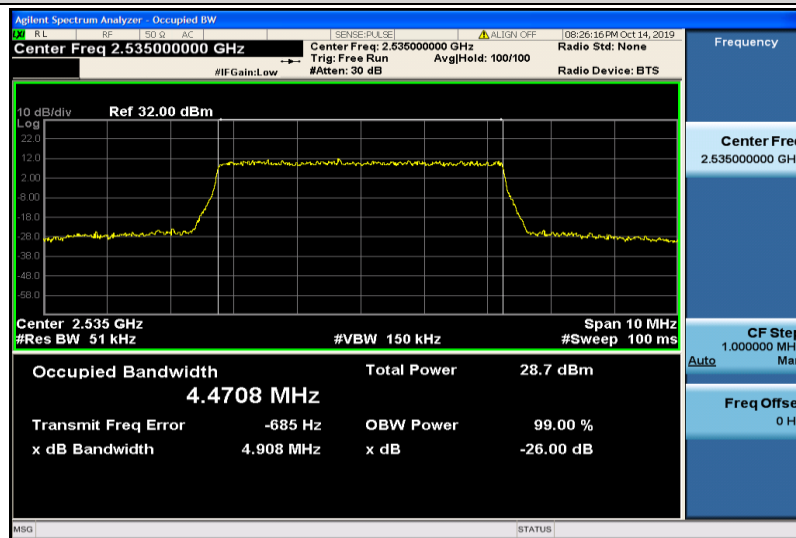
Band7-5MHz-QPSK-21100-25RB#0-4.4708
