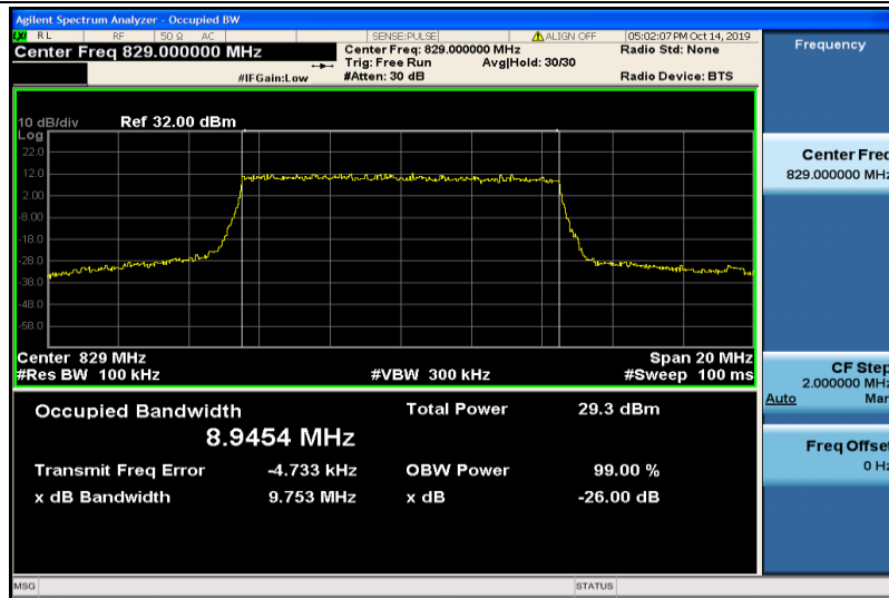
Band5-10MHz-QPSK-20450-50RB#0-8.9454
