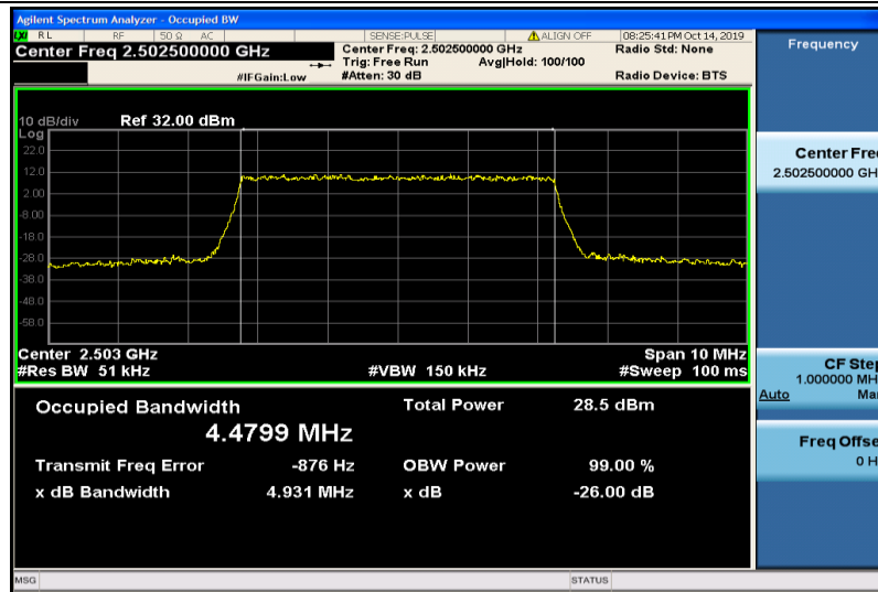
Band7-5MHz-QPSK-20775-25RB#0-4.4799
