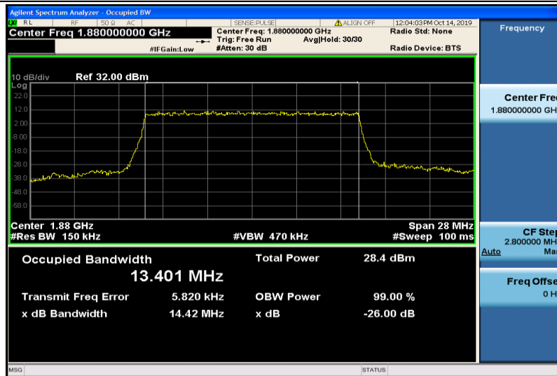
Band2-15MHz-16QAM-18900-75RB#0-13.401
