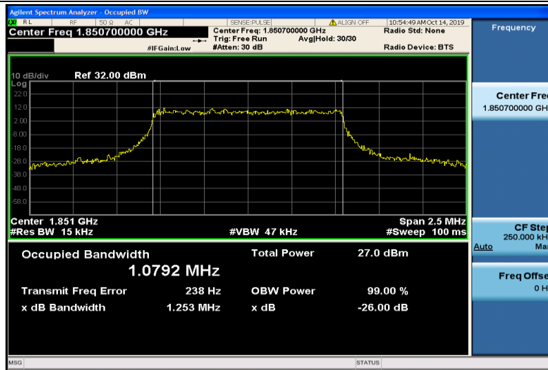
Band2-1.4MHz-16QAM-18607-6RB#0-1.0792
