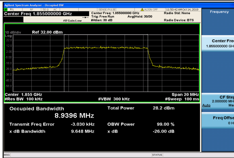
Band2-10MHz-16QAM-18650-50RB#0-8.9396
