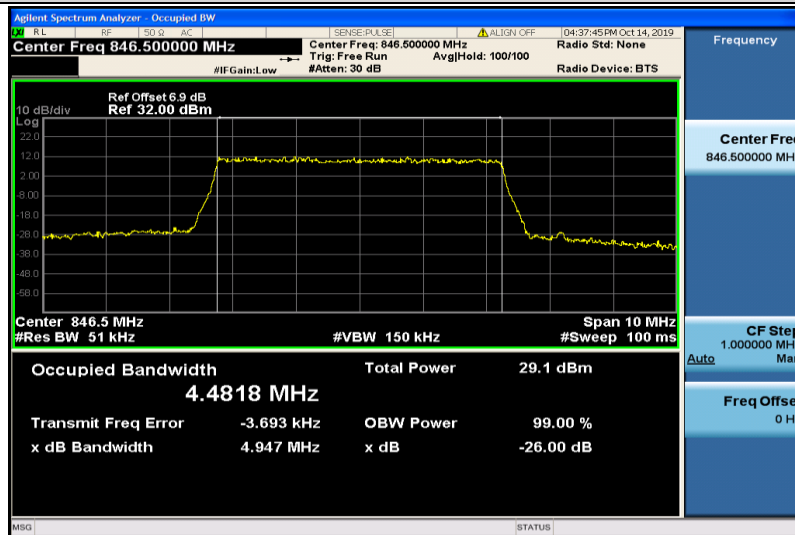
Band5-5MHz-QPSK-20625-25RB#0-4.4818
