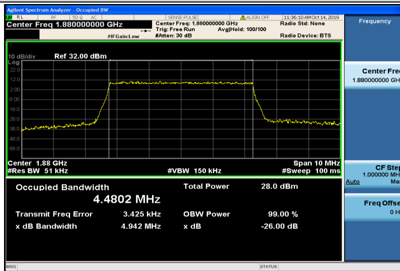
Band2-5MHz-16QAM-18900-25RB#0-4.4802
