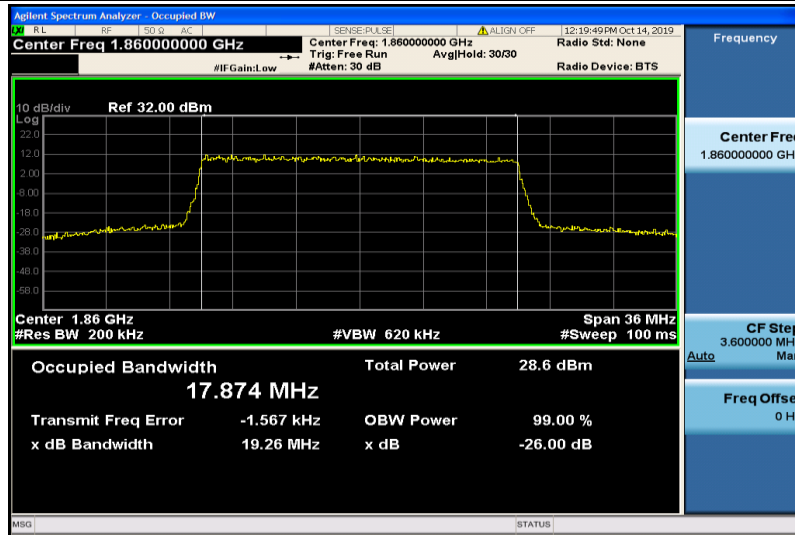
Band2-20MHz-16QAM-18700-100RB#0-17.874
