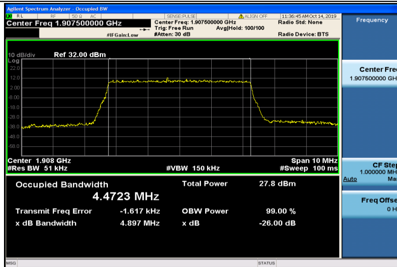
Band2-5MHz-16QAM-19175-25RB#0-4.4723
