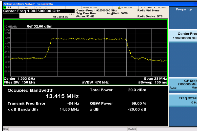
Band2-15MHz-QPSK-19125-75RB#0-13.415
