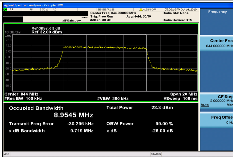
Band5-10MHz-16QAM-20600-50RB#0-8.9545
