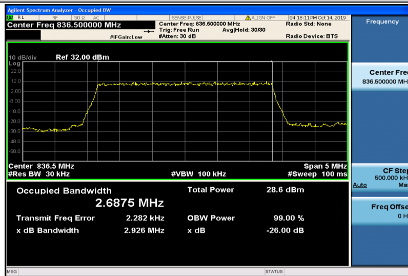
Band5-3MHz-QPSK-20525-15RB#0-2.6875
