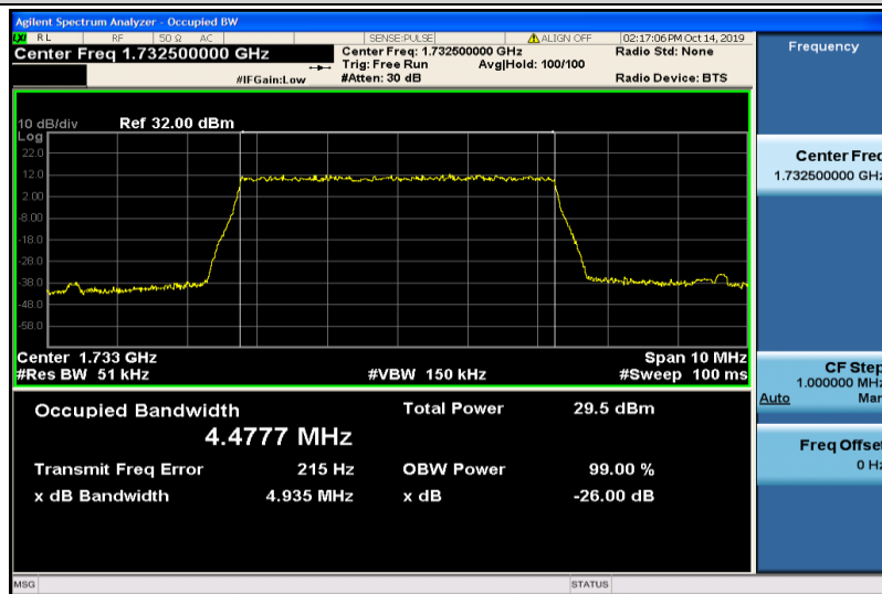
Band4-5MHz-QPSK-17325-25RB#0-4.4777
