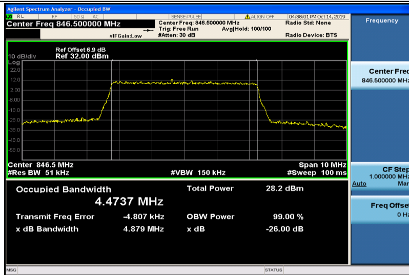
Band5-5MHz-16QAM-20625-25RB#0-4.4737
