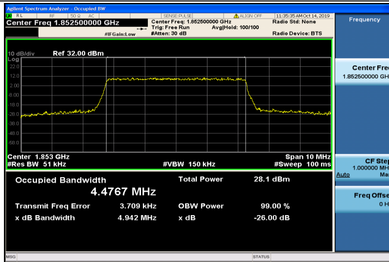
Band2-5MHz-16QAM-18625-25RB#0-4.4767
