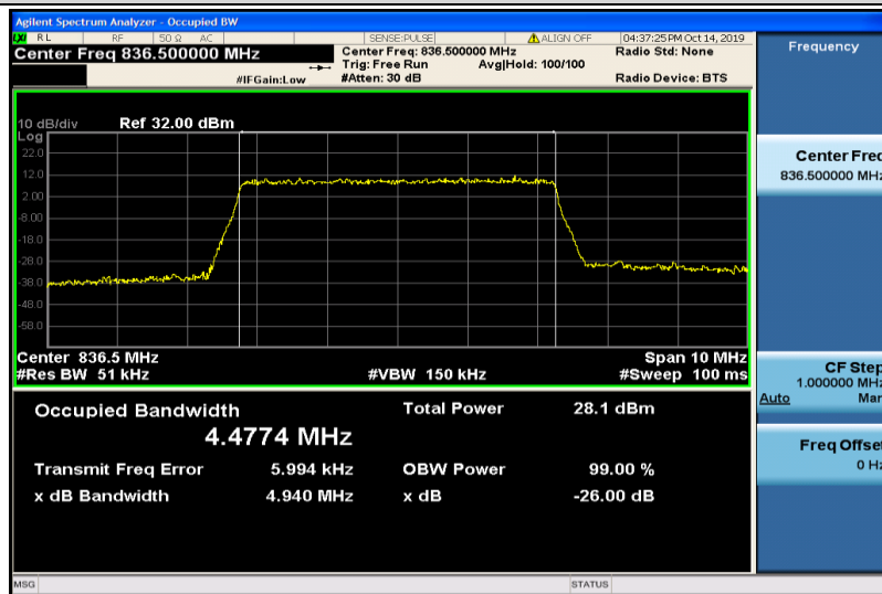
Band5-5MHz-16QAM-20525-25RB#0-4.4774
