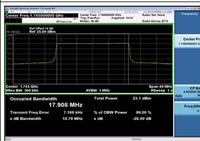
FDD66_MidRange_20_1745_QPSK
