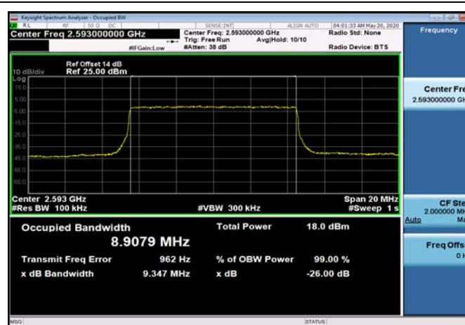
TDD41_MidRange_15_2593_QPSK
