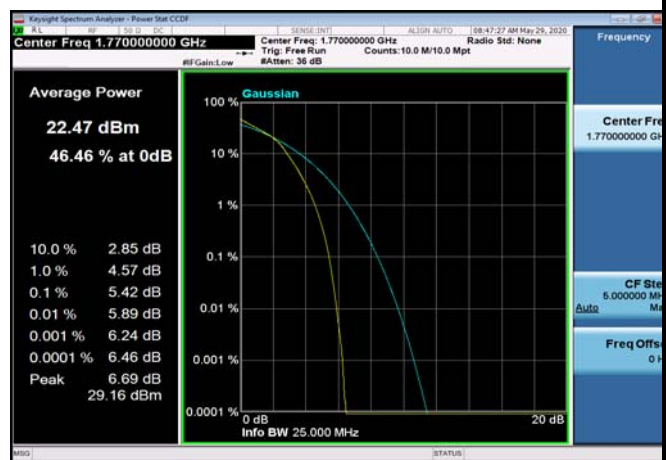
FDD66_HighRange_20MHz_1770_fullIRB_Q16
