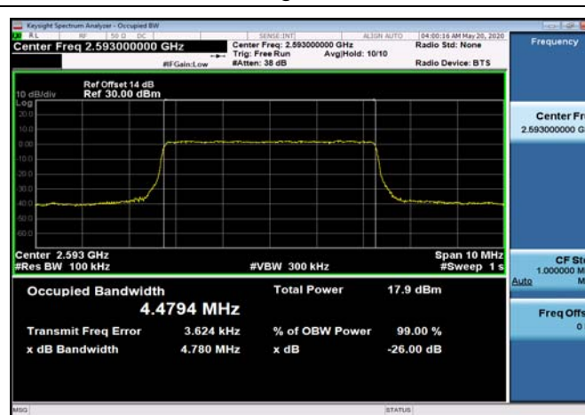
TDD41_MidRange_5_2593_QPSK
