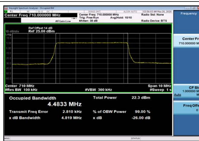
FDD17_MidRange_10_710_QPSK
