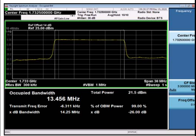
FDD04_MidRange_15MHz_1732.5MHz_Q16
