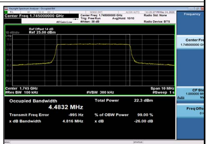
FDD66_MidRange_5_1745_Q16
