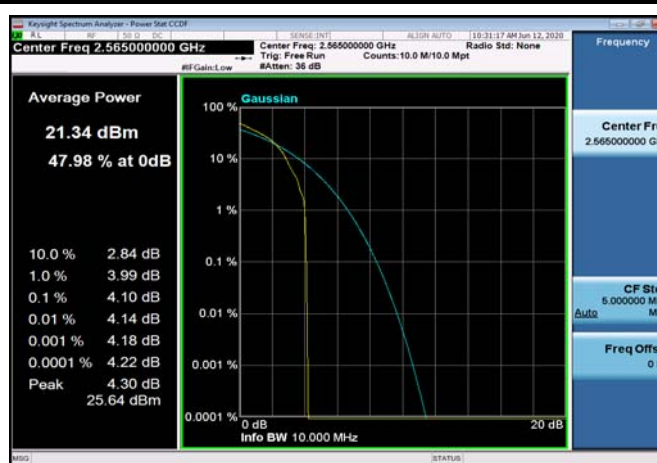
FDD07_HighRange_10MHz_2565_OneRB_high_Q16
