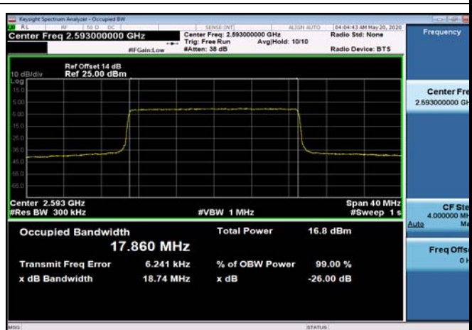
TDD41_MidRange_20_2593_Q16
