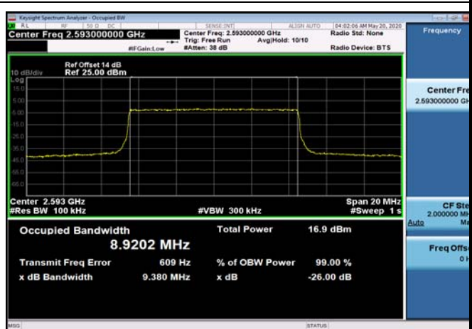
TDD41_MidRange_15_2593_Q16
