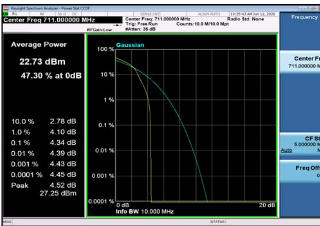
FDD12_HighRange_10MHz_711_OneRB _high_Q16
