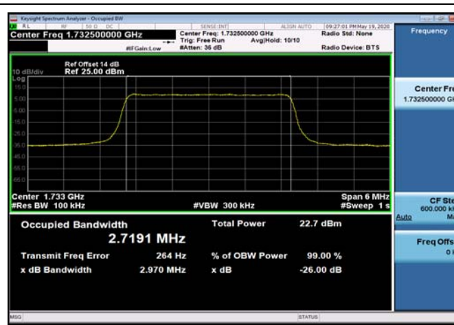
FDD04_MidRange_3MHz_1732.5MHz_QPSK
