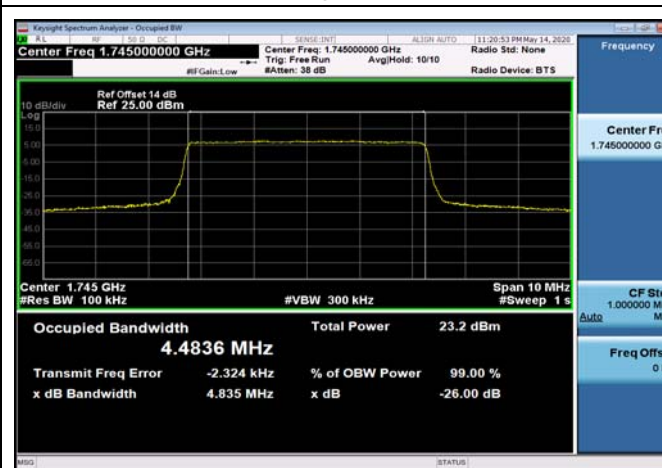
FDD66_MidRange_5_1745_QPSK
