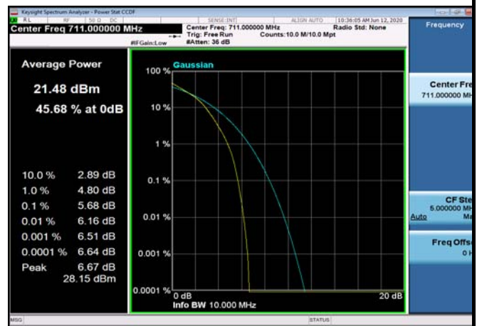
FDD12_HighRange_10MHz_711_fullRB _Q16
