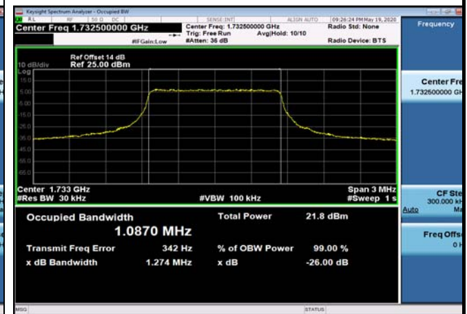
FDD04_MidRange_3MHz_1732.5MHz_Q16
