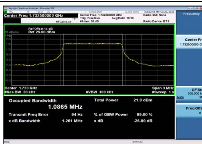
FDD04_MidRange_3_1732.5_QPSK
