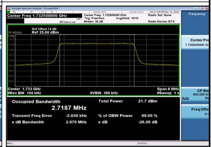
FDD04_MidRange_3MHz_1732.5MHz_Q16
