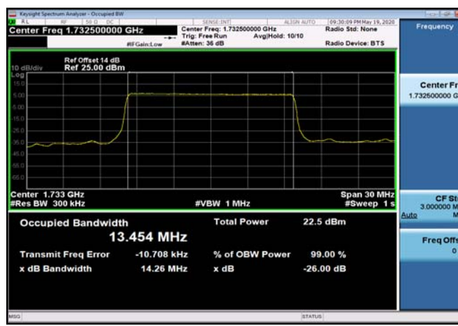
FDD04_MidRange_15MHz_1732.5MHz_QPSK
