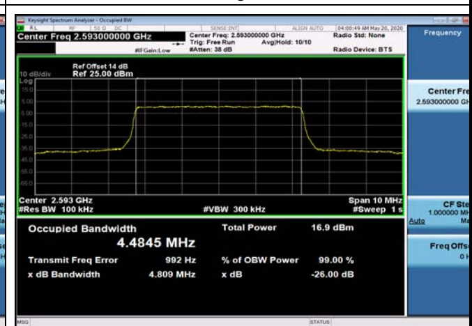
TDD41_MidRange_5_2593_Q16
