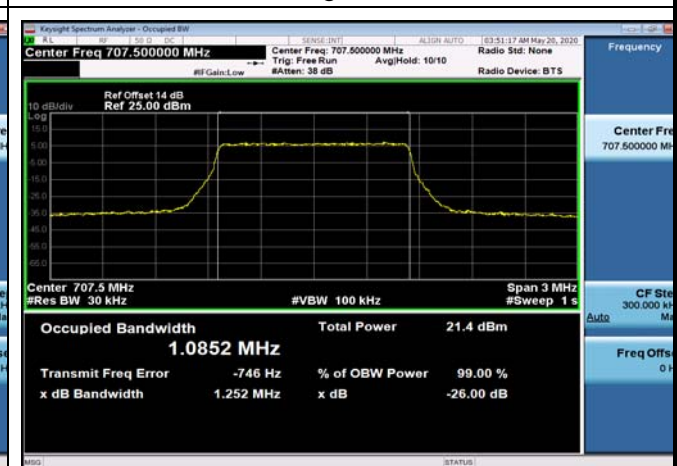
FDD12_MidRange_1.4_707.5_Q16
