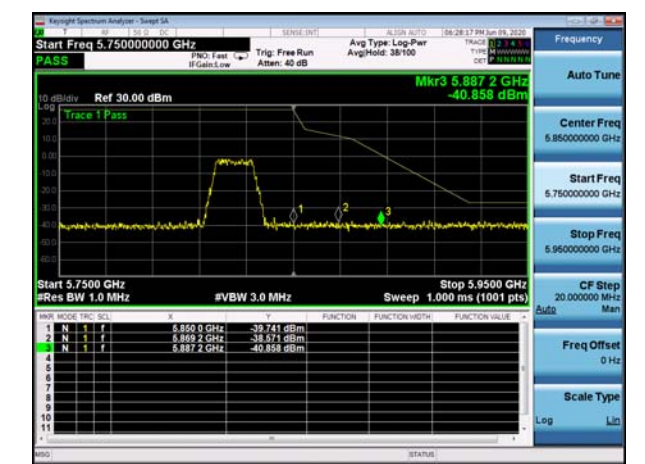
U-NII-3 ,Plot 1,Band Edge-802.11a(20M Hz),5825MHz
