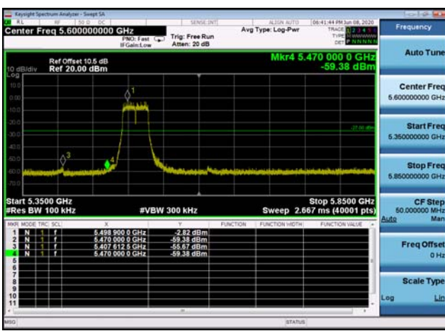
U-NII-2c ,Plot 1, Band Edge-802.11a(40 MHz),5510MHz
