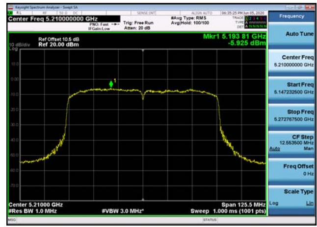
U-NII-1 Power spectral density-802.11 ac(80MHz),5210MHz
