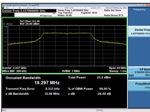
99% Bandwidth-802.11g,2437MHz
