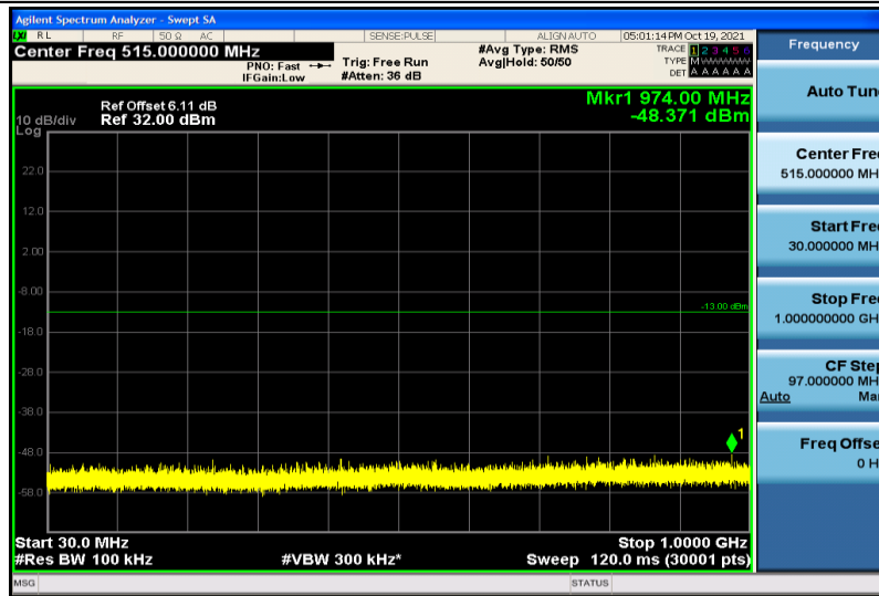
Band66-1.4MHz-16QAM-132322-1RB#0-30~1000MHz
