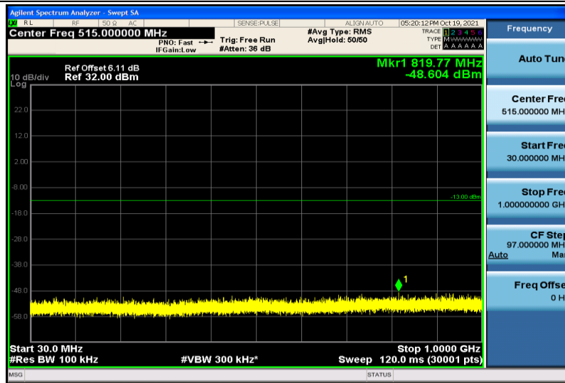
Band66-5MHz-16QAM-132322-1RB#0-30~1000MHz
