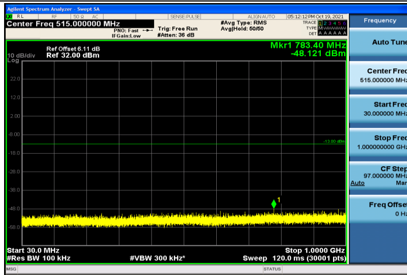
Band66-3MHz-16QAM-132322-1RB#0-30~1000MHz
