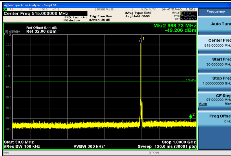
Band17-10MHz-16QAM-23790-1RB#0-30~1000MHz
