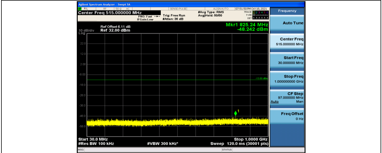
Band2-1.4MHz-QPSK-18607-1RB#0-30~1000MHz
