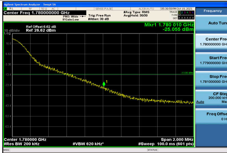
Band66-20MHz-16QAM-132572-1RB#99
