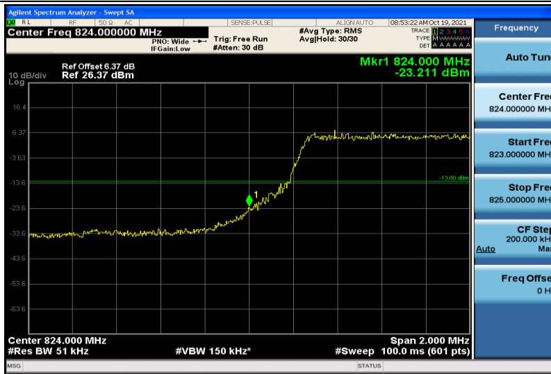
Band5-5MHz-QPSK-20425-25RB#0
