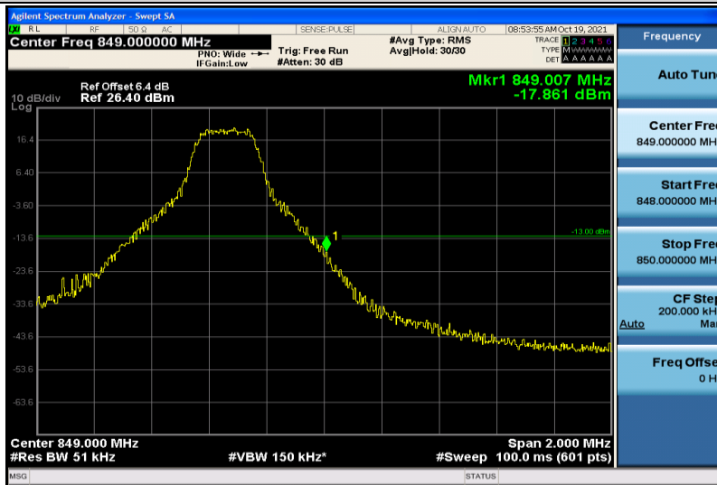
Band5-5MHz-QPSK-20625-1RB#24
