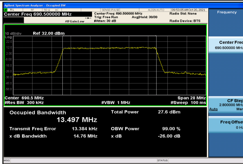
Band71-15MHz-16QAM-133397-75RB#0-13.497
