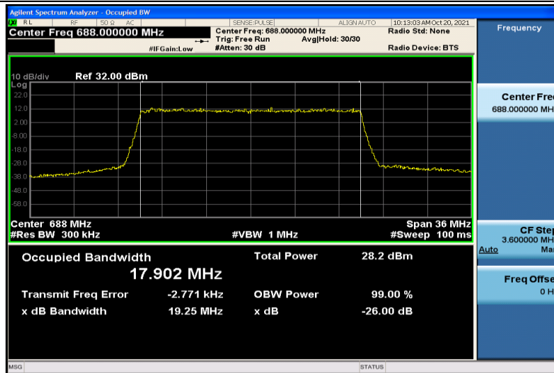
Band71-20MHz-QPSK-133372-100RB#0-17.902
