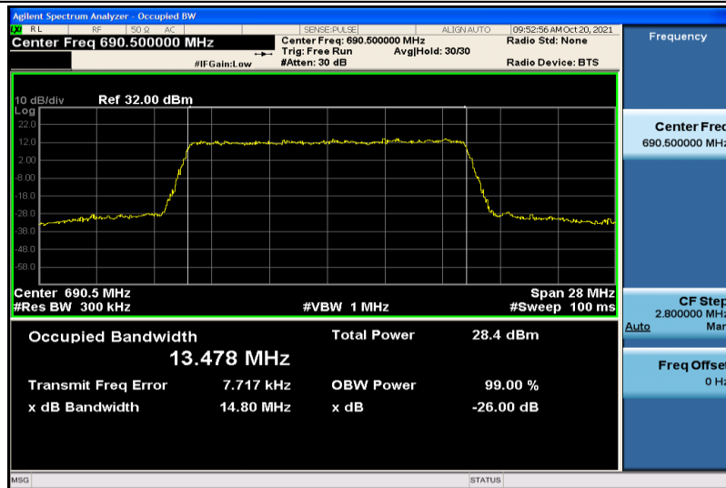
Band71-15MHz-QPSK-133397-75RB#0-13.478
