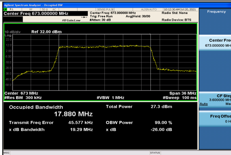
Band71-20MHz-16QAM-133222-100RB#0-17.880
