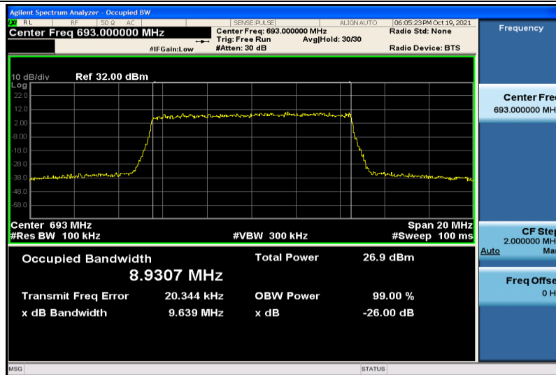
Band71-10MHz-16QAM-133422-50RB#0-8.9307
