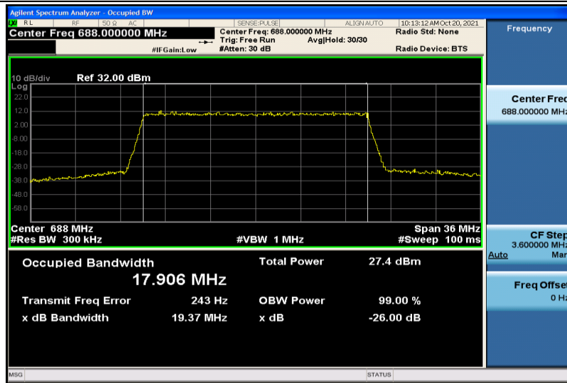
Band71-20MHz-16QAM-133372-100RB#0-17.906
