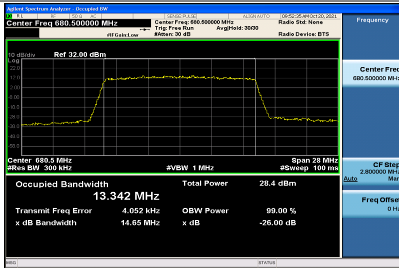
Band71-15MHz-QPSK-133297-75RB#0-13.342
