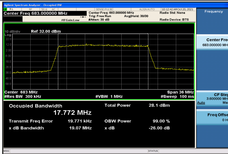
Band71-20MHz-QPSK-133322-100RB#0-17.772
