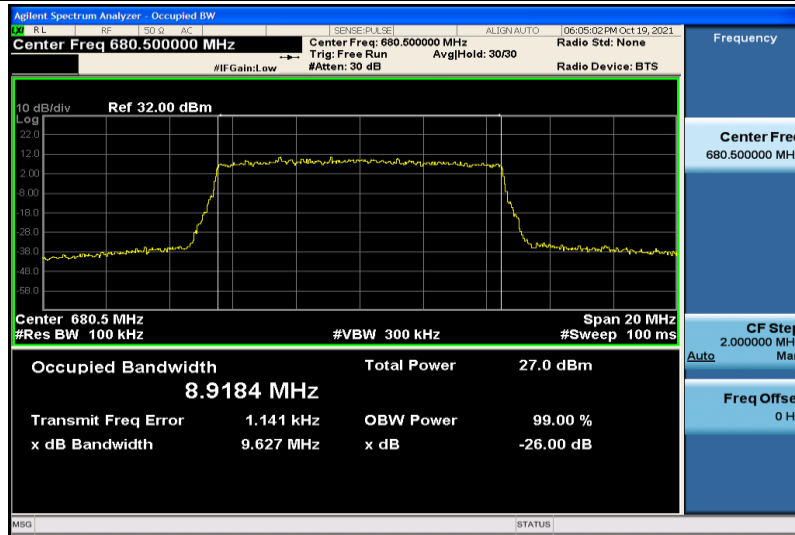
Band71-10MHz-16QAM-133297-50RB#0-8.9184
