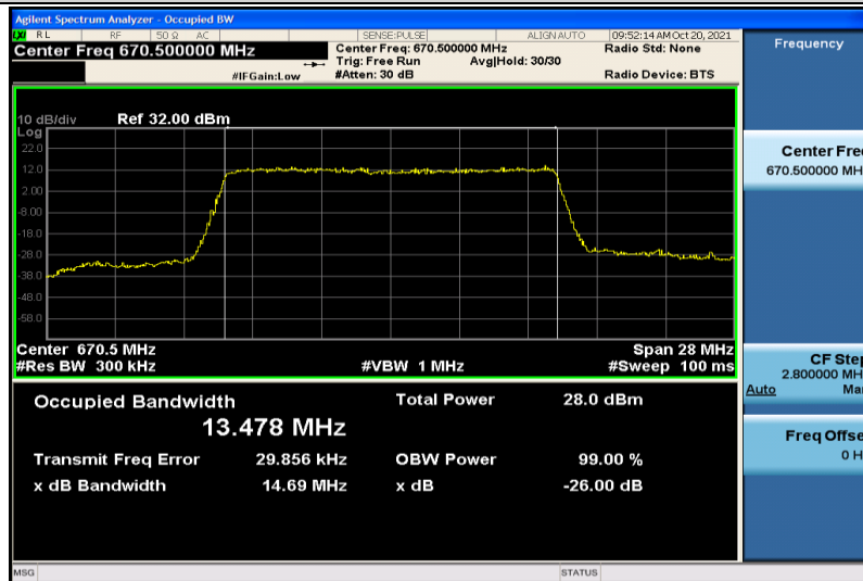
Band71-15MHz-QPSK-133197-75RB#0-13.478
