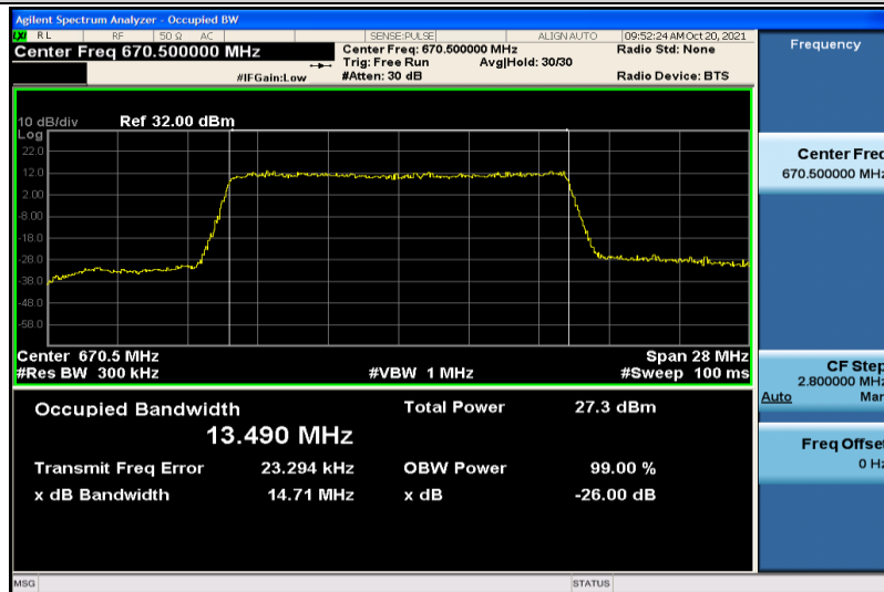
Band71-15MHz-16QAM-133197-75RB#0-13.490
