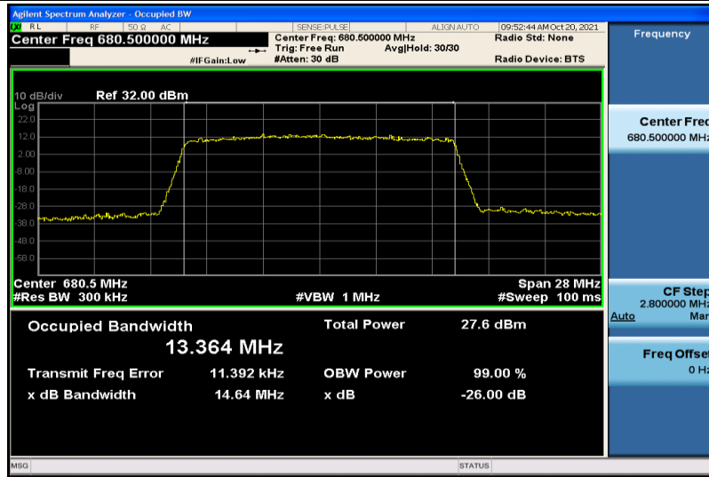
Band71-15MHz-16QAM-133297-75RB#0-13.364
