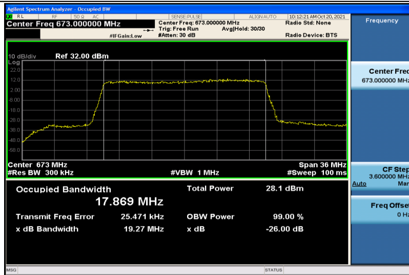
Band71-20MHz-QPSK-133222-100RB#0-17.869
