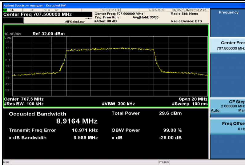
Band12-10MHz-16QAM-23095-50RB#0-8.9164
