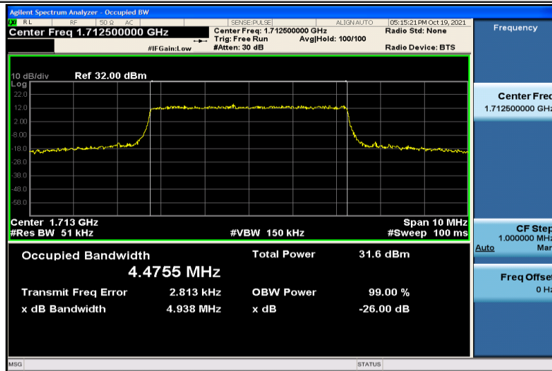
Band66-5MHz-QPSK-131997-25RB#0-4.4755
