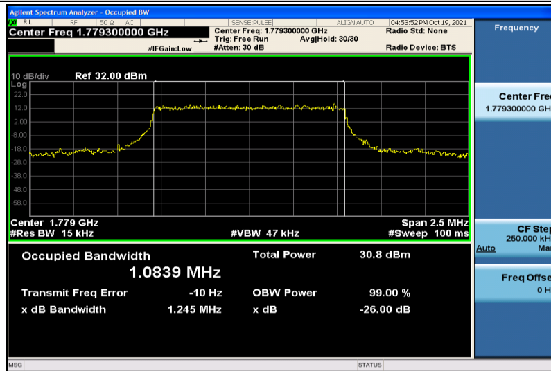
Band66-1.4MHz-QPSK-132665-6RB#0-1.0839
