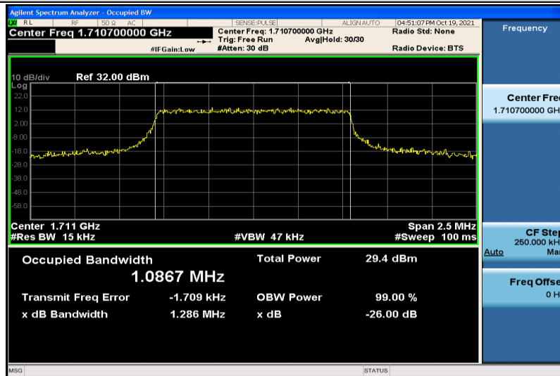
Band66-1.4MHz-16QAM-131979-6RB#0-1.0867
