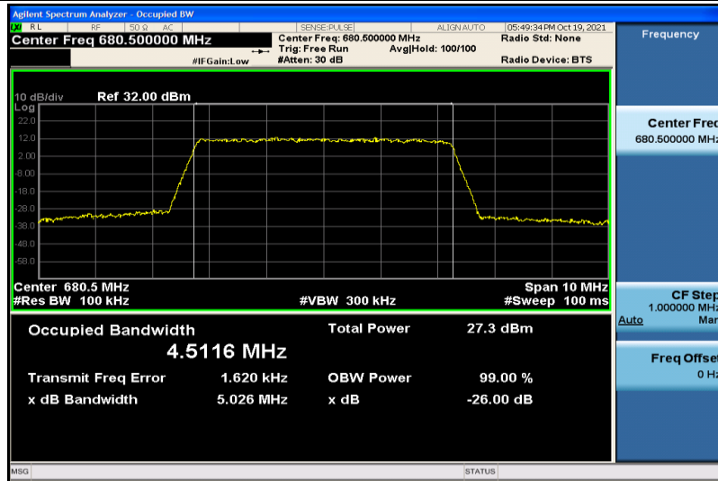
Band71-5MHz-16QAM-133297-25RB#0-4.5116
