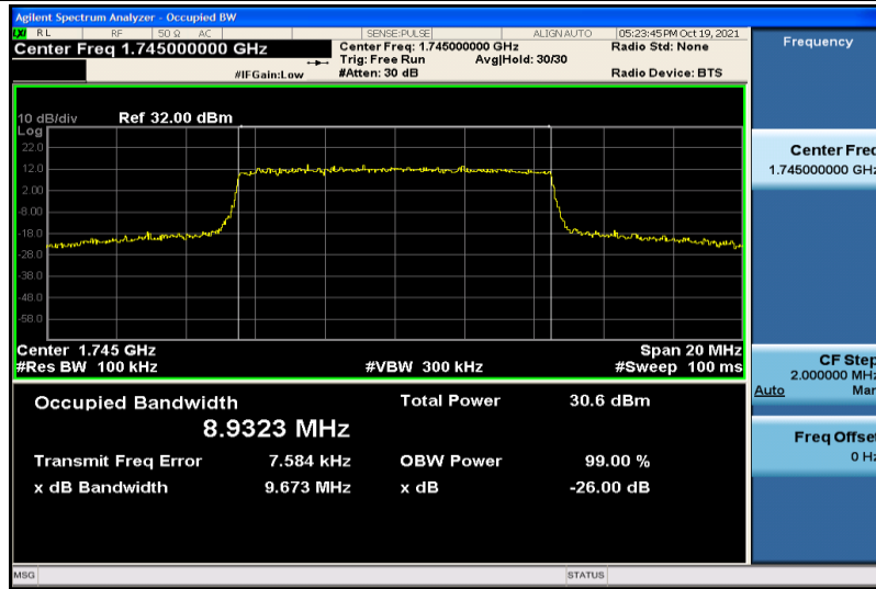
Band66-10MHz-16QAM-132322-50RB#0-8.9323
