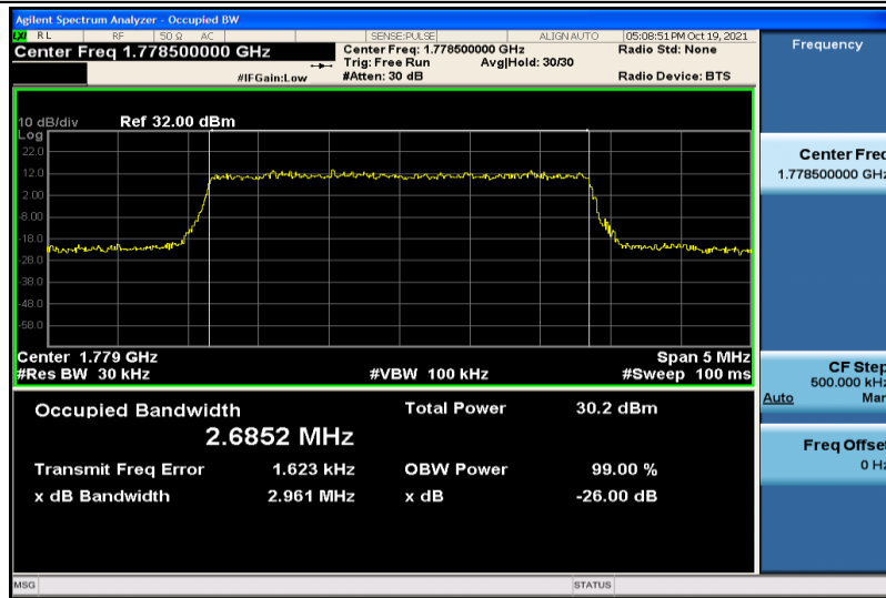
Band66-3MHz-16QAM-132657-15RB#0-2.6852
