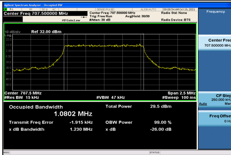
Band12-1.4MHz-QPSK-23095-6RB#0-1.0802
