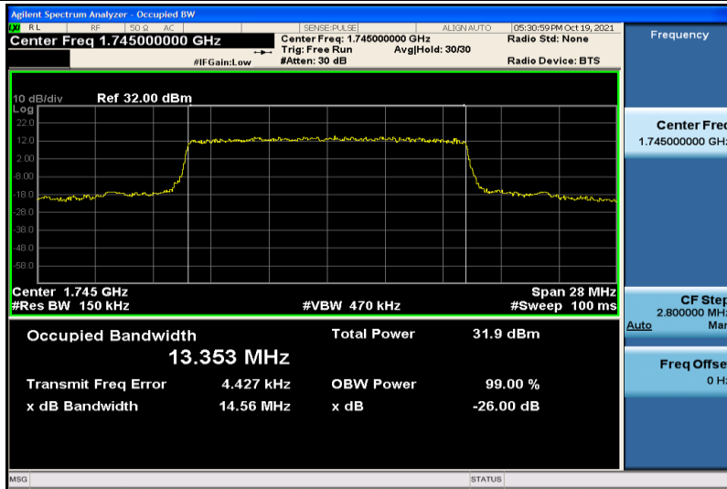
Band66-15MHz-QPSK-132322-75RB#0-13.353
