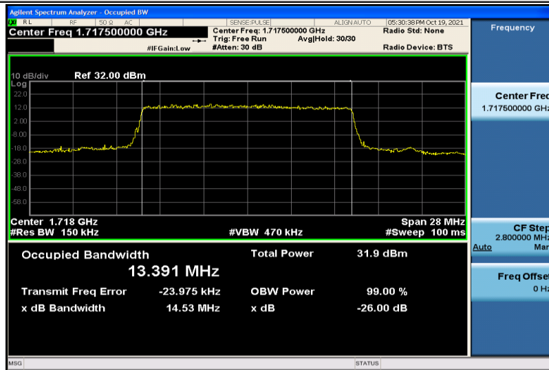
Band66-15MHz-QPSK-132047-75RB#0-13.391
