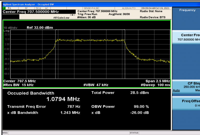
Band12-1.4MHz-16QAM-23095-6RB#0-1.0794
