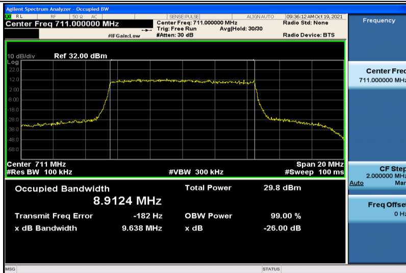
Band12-10MHz-16QAM-23130-50RB#0-8.9124
