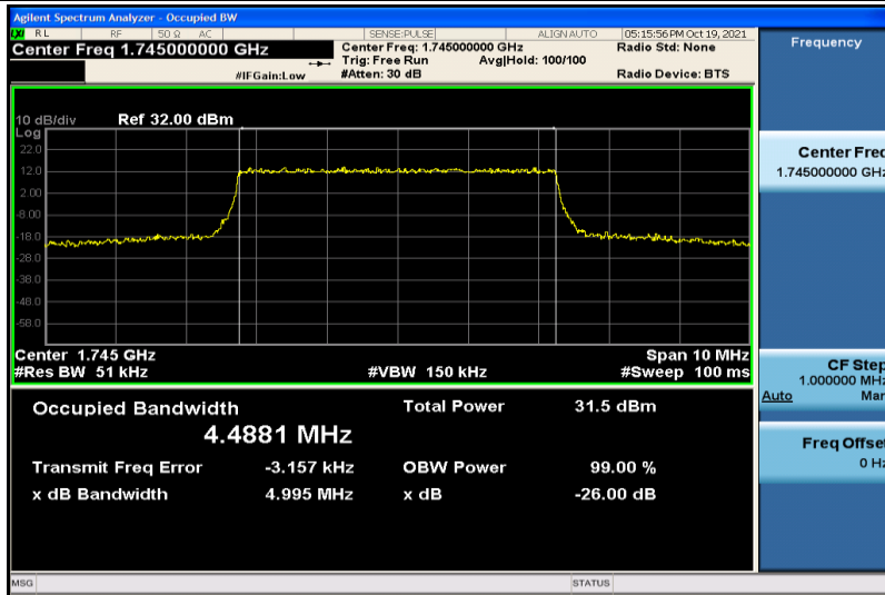
Band66-5MHz-QPSK-132322-25RB#0-4.4881
