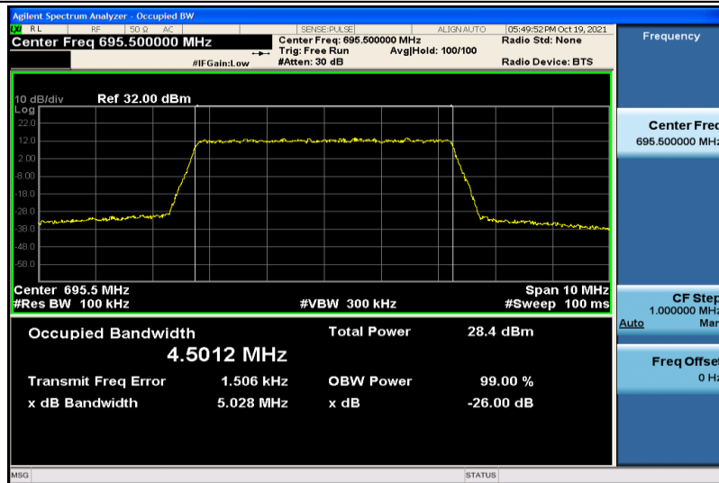
Band71-5MHz-QPSK-133447-25RB#0-4.5012
