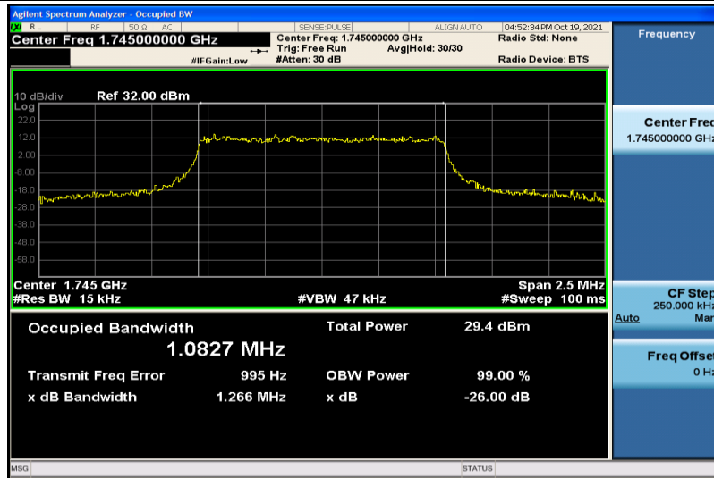
Band66-1.4MHz-16QAM-132322-6RB#0-1.0827
