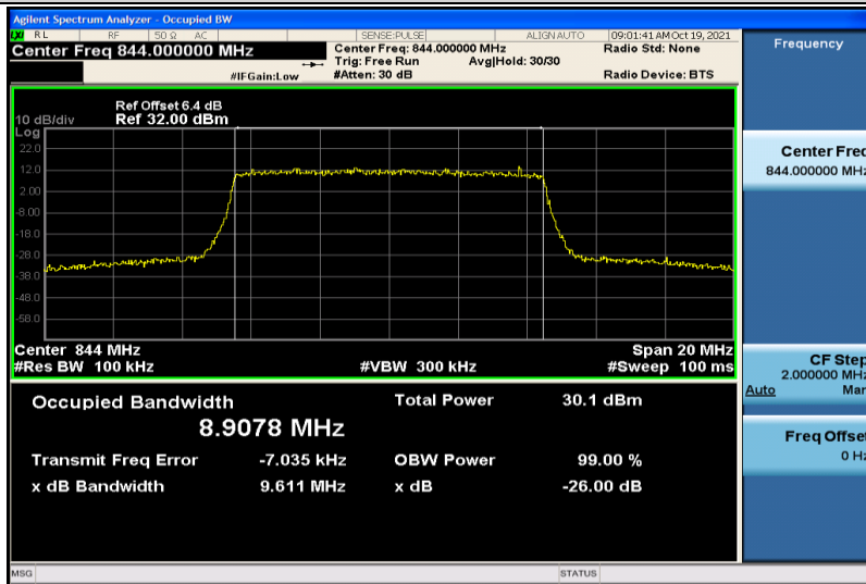
Band5-10MHz-16QAM-20600-50RB#0-8.9078
