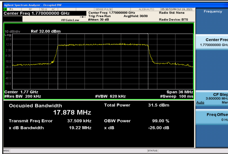
Band66-20MHz-16QAM-132572-100RB#0-17.878
