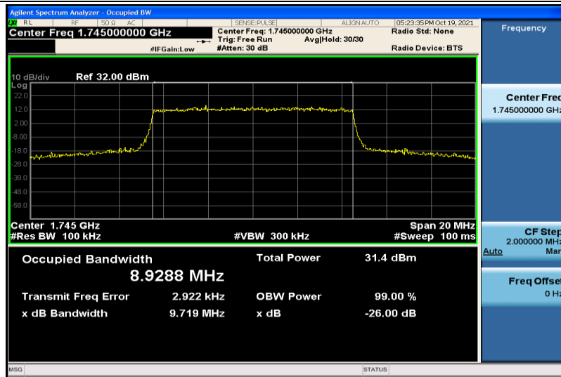
Band66-10MHz-QPSK-132322-50RB#0-8.9288
