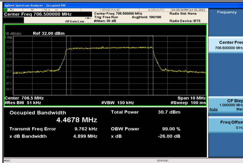
Band17-5MHz-QPSK-23755-25RB#0-4.4678
