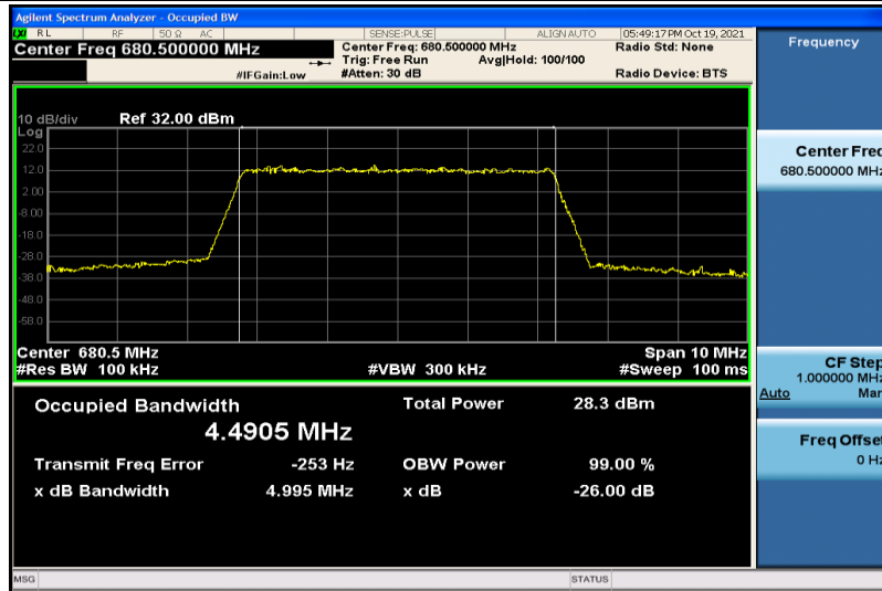
Band71-5MHz-QPSK-133297-25RB#0-4.4905
