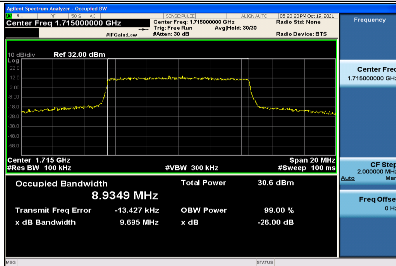
Band66-10MHz-16QAM-132022-50RB#0-8.9349
