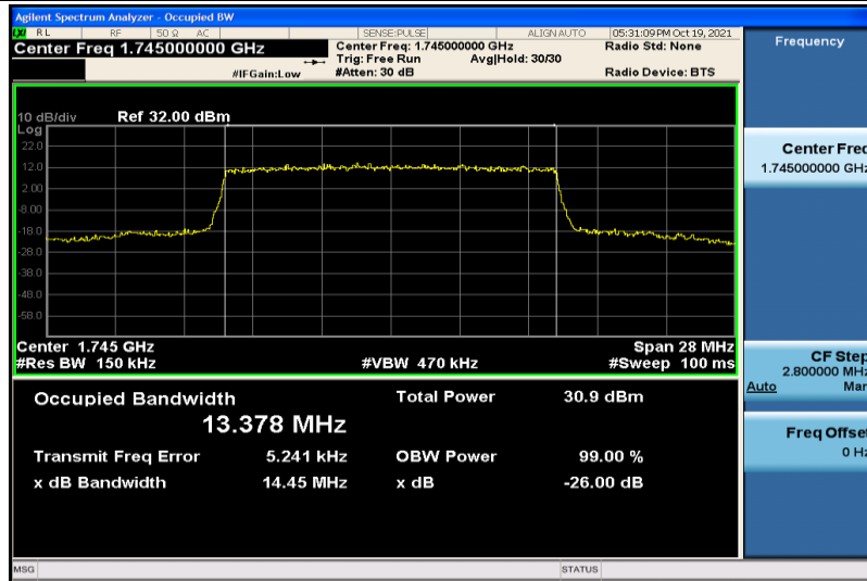
Band66-15MHz-16QAM-132322-75RB#0-13.378
