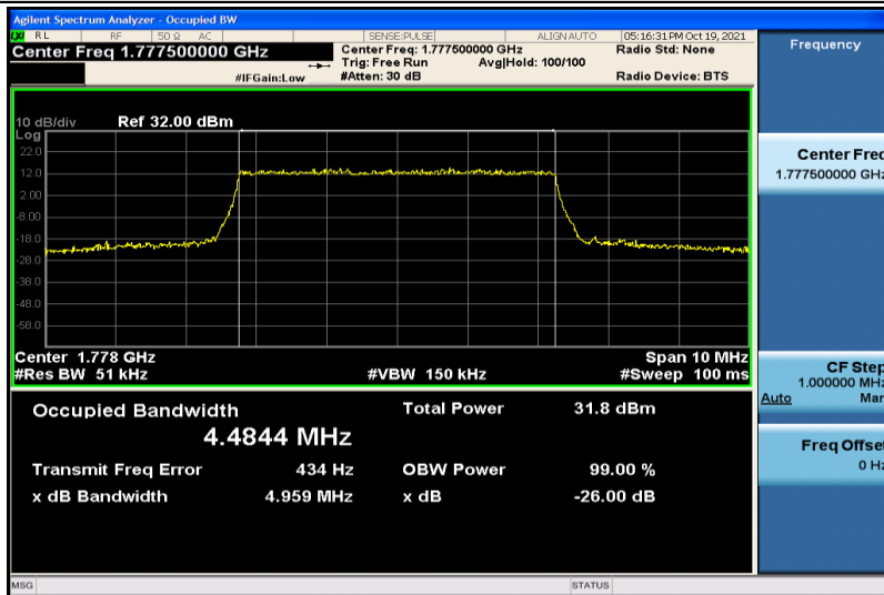
Band66-5MHz-QPSK-132647-25RB#0-4.4844
