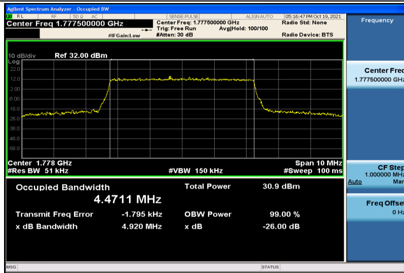
Band66-5MHz-16QAM-132647-25RB#0-4.4711
