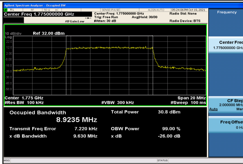
Band66-10MHz-16QAM-132622-50RB#0-8.9235
