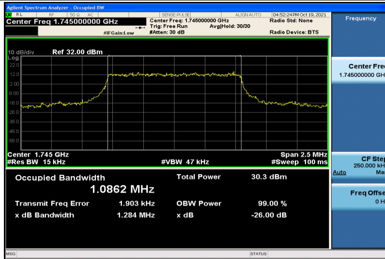
Band66-1.4MHz-QPSK-132322-6RB#0-1.0862
