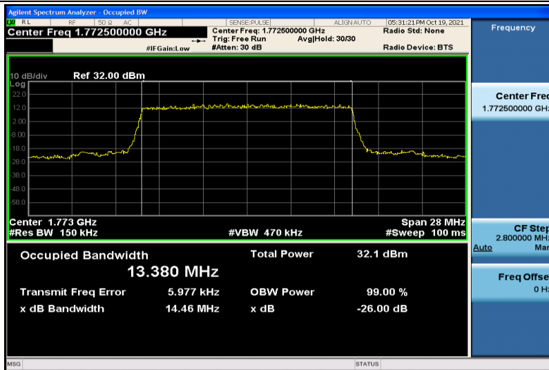
Band66-15MHz-QPSK-132597-75RB#0-13.380
