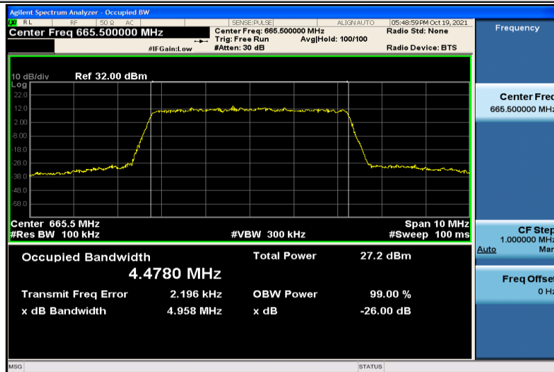
Band71-5MHz-16QAM-133147-25RB#0-4.4780
