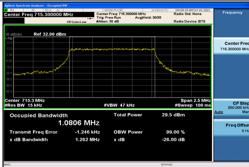
Band12-1.4MHz-QPSK-23173-6RB#0-1.0806
