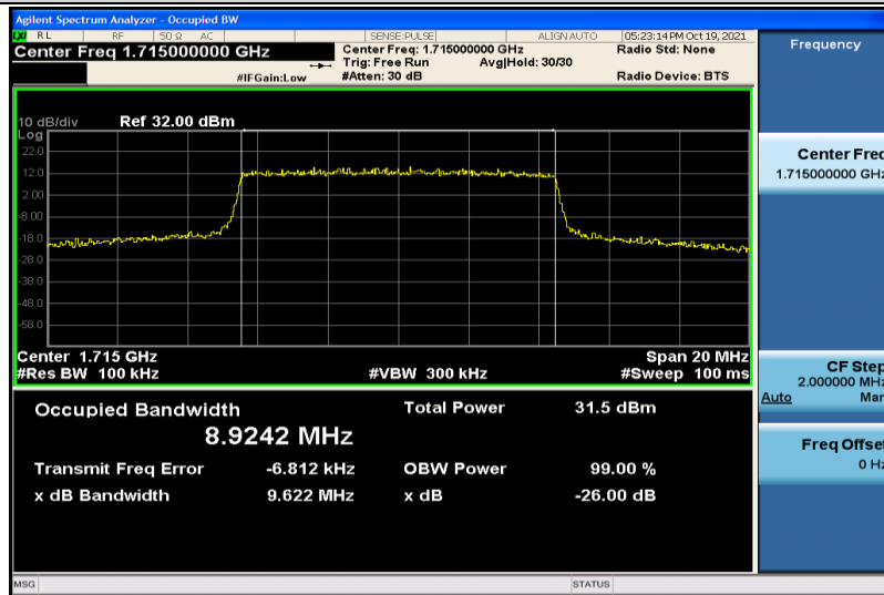
Band66-10MHz-QPSK-132022-50RB#0-8.9242
