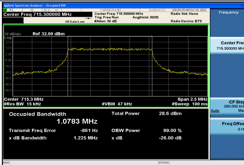
Band12-1.4MHz-16QAM-23173-6RB#0-1.0783
