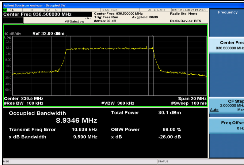
Band5-10MHz-16QAM-20525-50RB#0-8.9346
