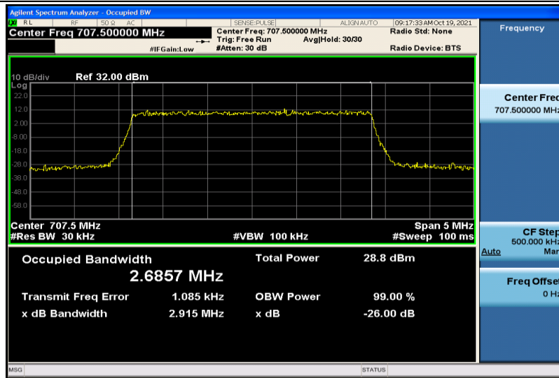
Band12-3MHz-16QAM-23095-15RB#0-2.6857
