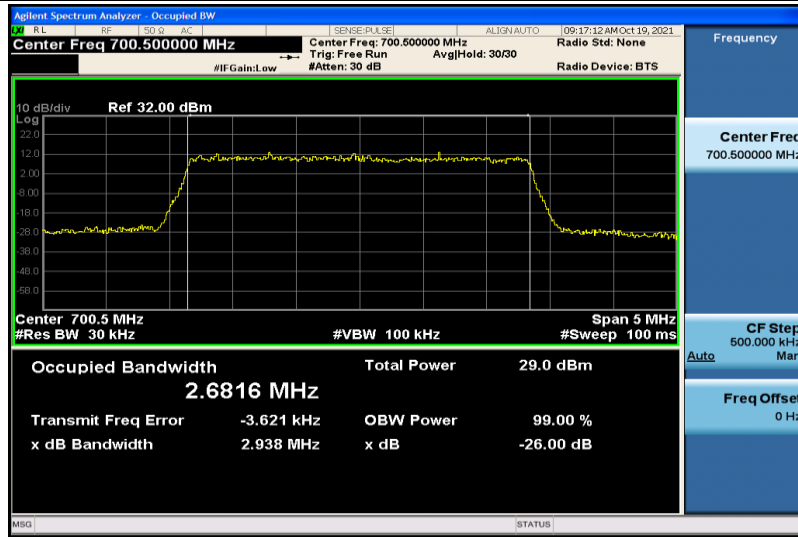
Band12-3MHz-16QAM-23025-15RB#0-2.6816
