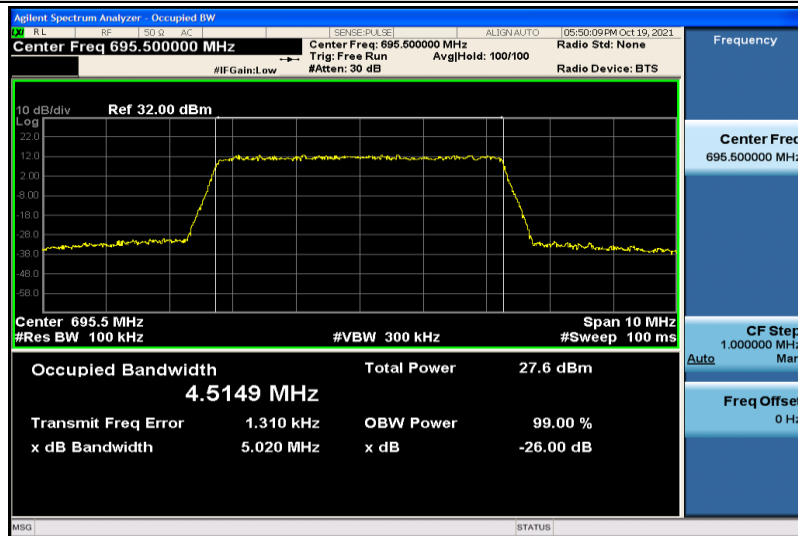
Band71-5MHz-16QAM-133447-25RB#0-4.5149
