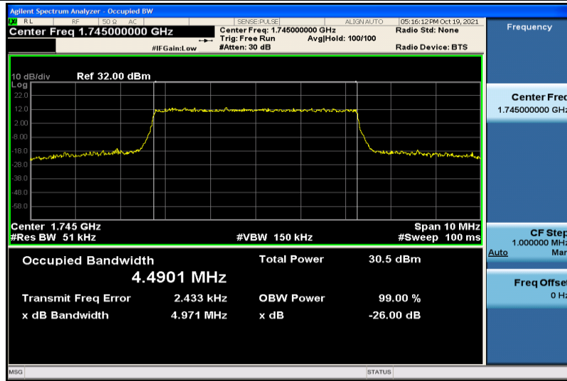
Band66-5MHz-16QAM-132322-25RB#0-4.4901
