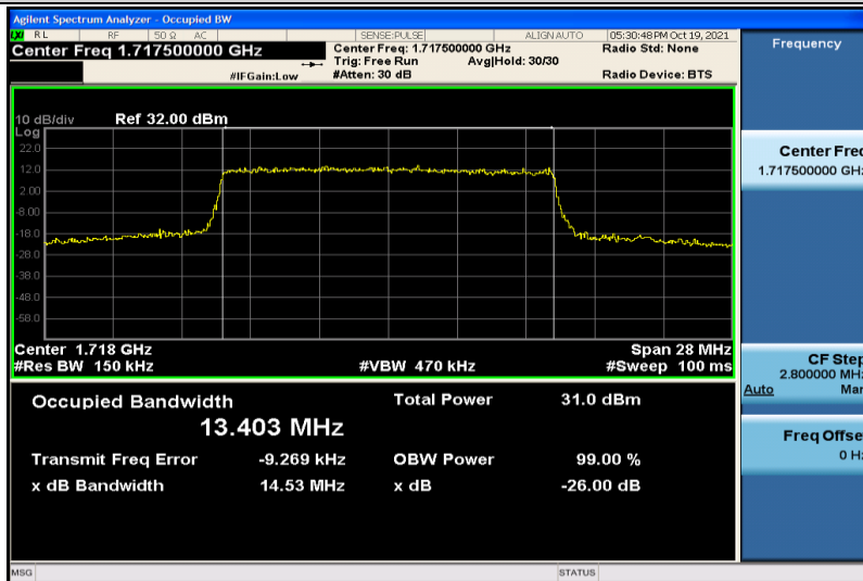
Band66-15MHz-16QAM-132047-75RB#0-13.403
