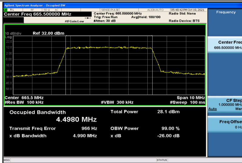
Band71-5MHz-QPSK-133147-25RB#0-4.4980
