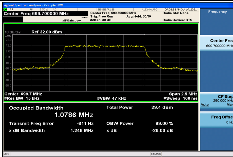
Band12-1.4MHz-QPSK-23017-6RB#0-1.0786
