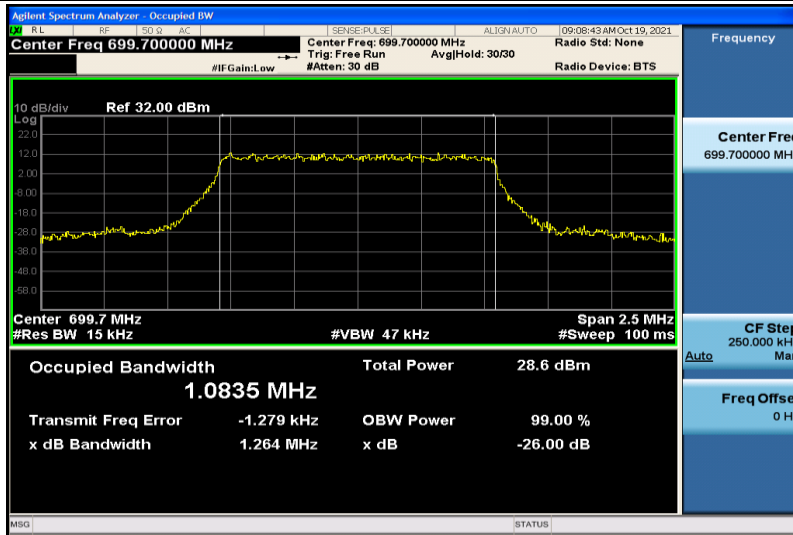
Band12-1.4MHz-16QAM-23017-6RB#0-1.0835
