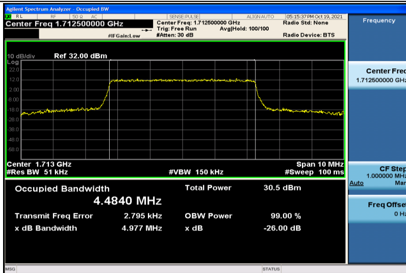
Band66-5MHz-16QAM-131997-25RB#0-4.4840
