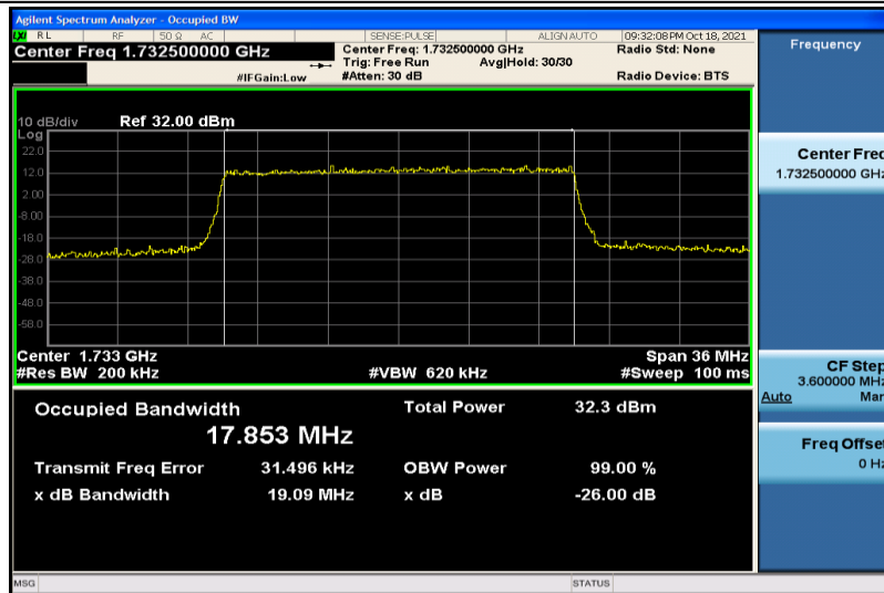
Band4-20MHz-QPSK-20175-100RB#0-17.853
