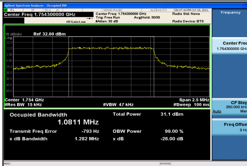
Band4-1.4MHz-QPSK-20393-6RB#0-1.0811
