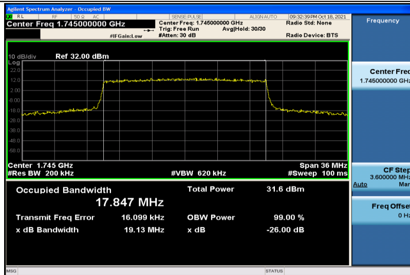
Band4-20MHz-16QAM-20300-100RB#0-17.847
