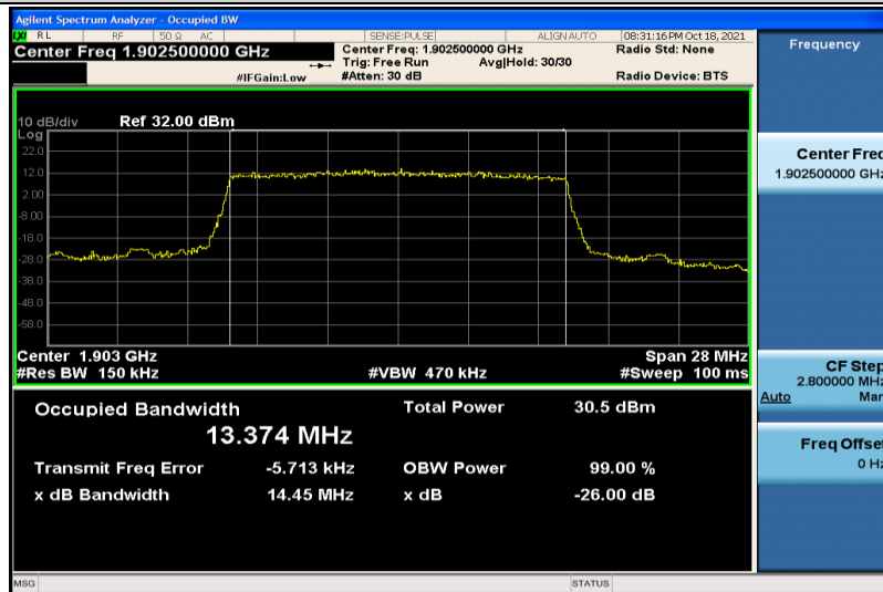
Band2-15MHz-QPSK-19125-75RB#0-13.374
