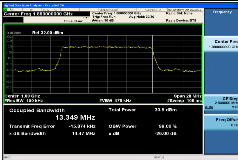
Band2-15MHz-QPSK-18900-75RB#0-13.349
