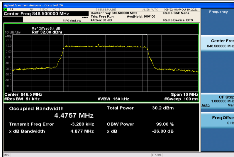
Band5-5MHz-16QAM-20625-25RB#0-4.4757
