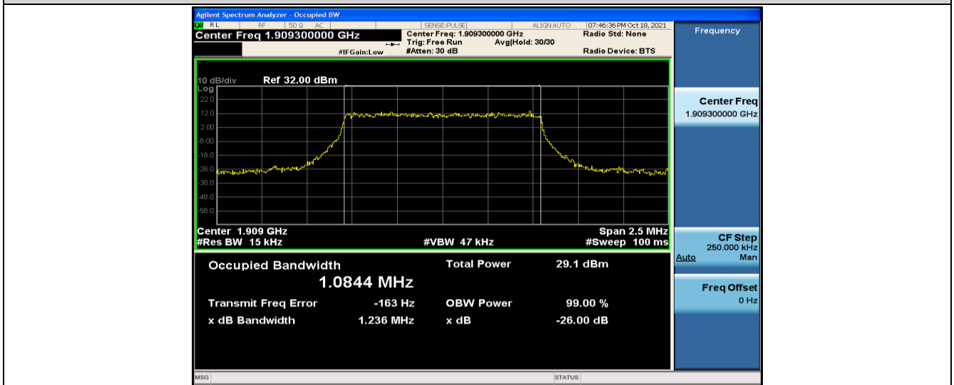
Band2-1.4MHz-QPSK-19193-6RB#0-1.0844
