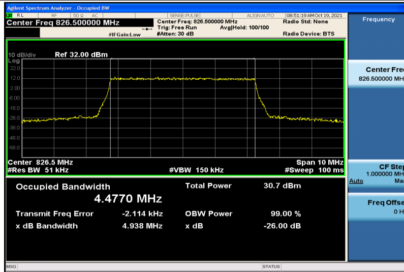
Band5-5MHz-QPSK-20425-25RB#0-4.4770
