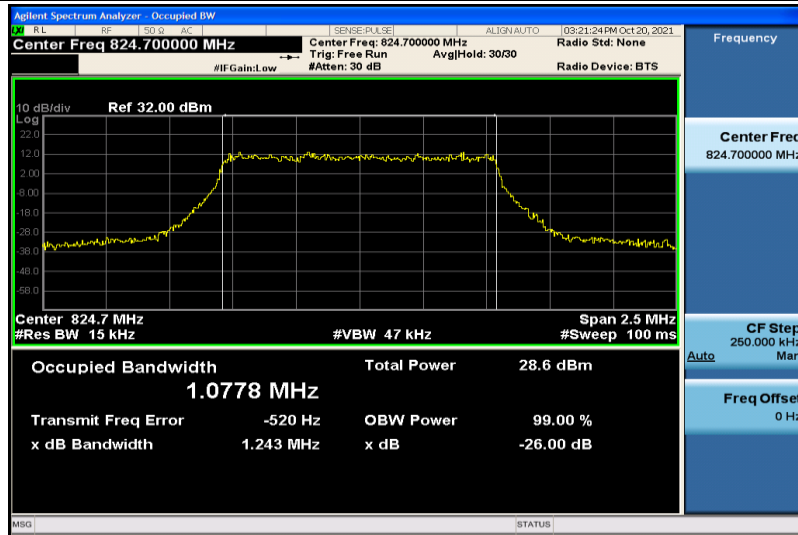
Band5-1.4MHz-16QAM-20407-6RB#0-1.0778
