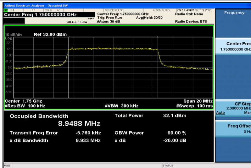
Band4-10MHz-QPSK-20350-50RB#0-8.9488
