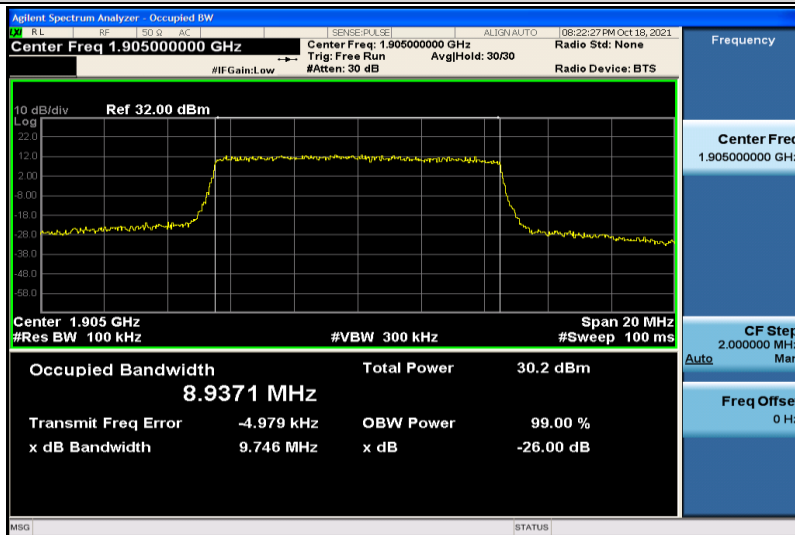
Band2-10MHz-QPSK-19150-50RB#0-8.9371
