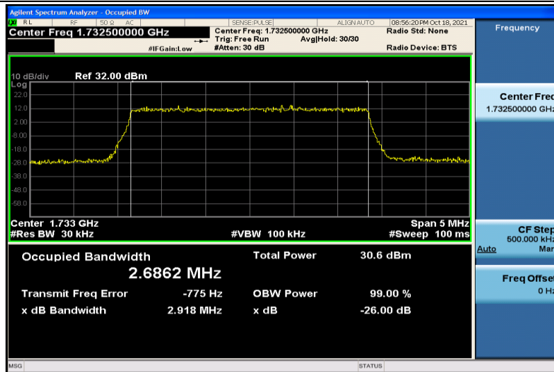
Band4-3MHz-16QAM-20175-15RB#0-2.6862
