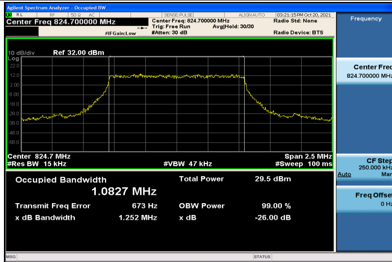
Band5-1.4MHz-QPSK-20407-6RB#0-1.0827
