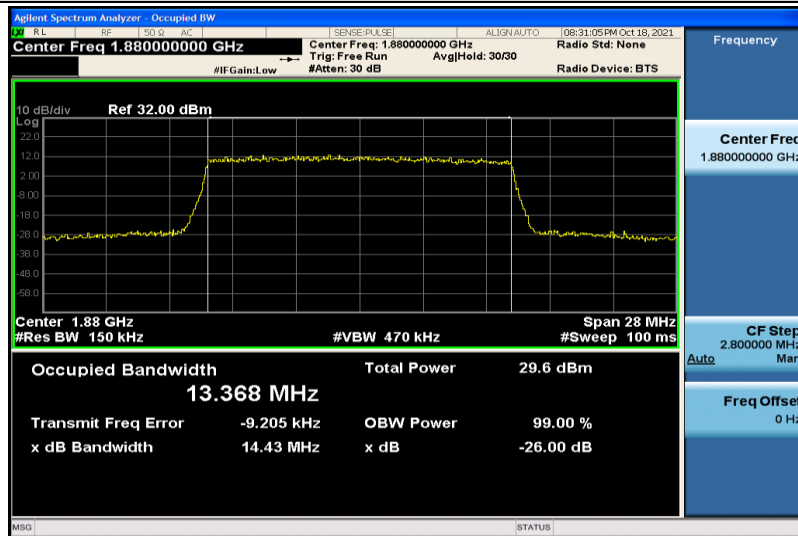
Band2-15MHz-16QAM-18900-75RB#0-13.368
