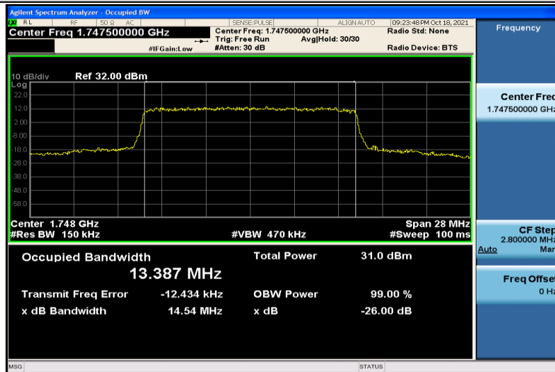
Band4-15MHz-16QAM-20325-75RB#0-13.387
