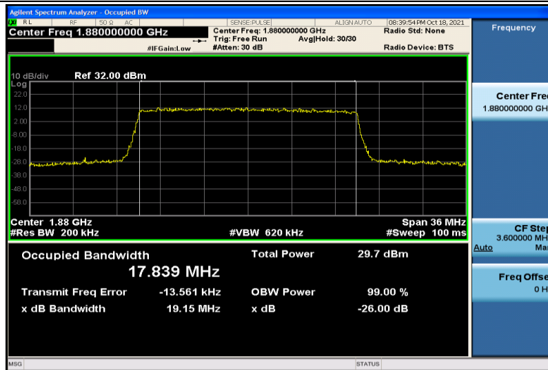
Band2-20MHz-16QAM-18900-100RB#0-17.839
