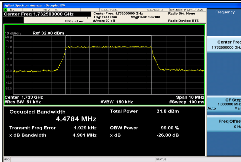
Band4-5MHz-QPSK-20175-25RB#0-4.4784
