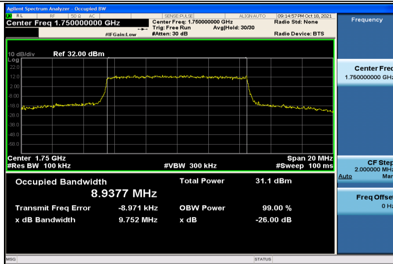
Band4-10MHz-16QAM-20350-50RB#0-8.9377
