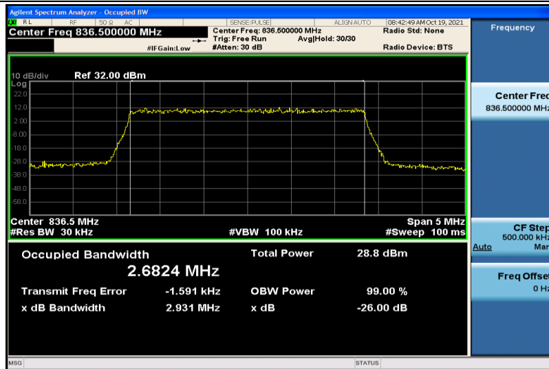
Band5-3MHz-QPSK-20525-15RB#0-2.6824
