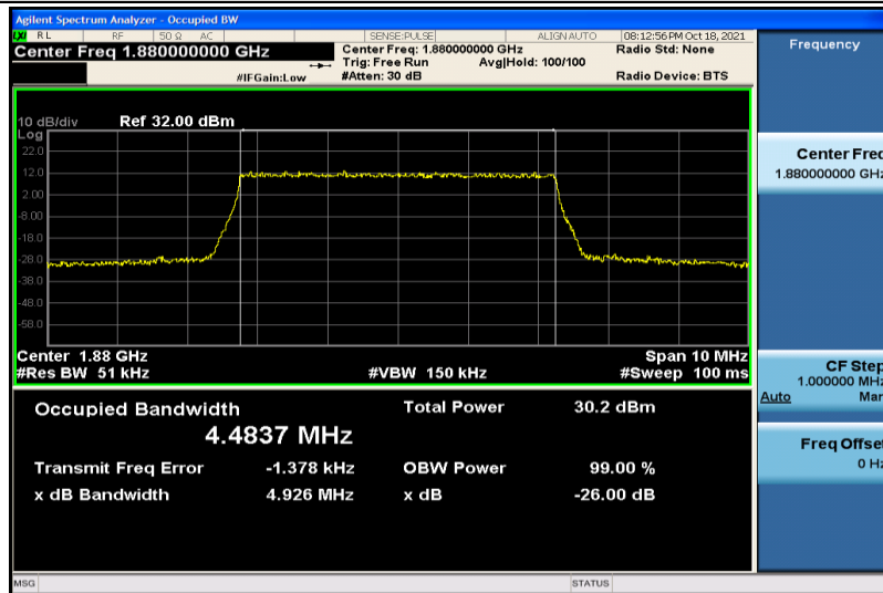
Band2-5MHz-QPSK-18900-25RB#0-4.4837
