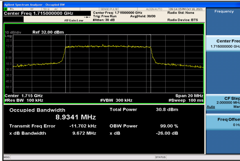
Band4-10MHz-16QAM-20000-50RB#0-8.9341
