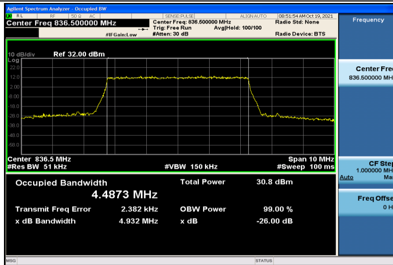
Band5-5MHz-QPSK-20525-25RB#0-4.4873
