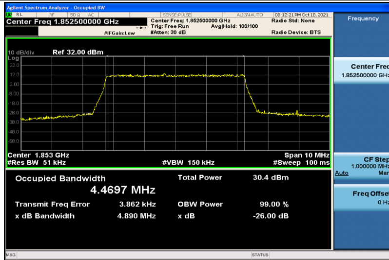
Band2-5MHz-QPSK-18625-25RB#0-4.4697
