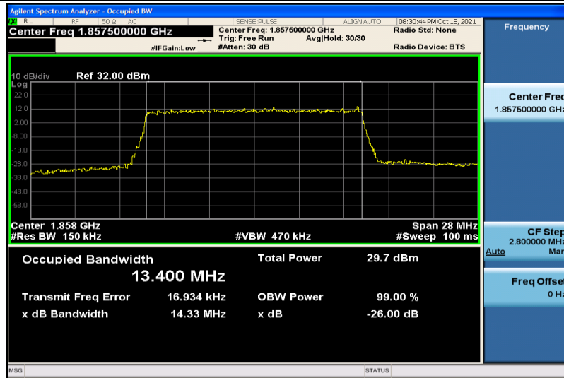
Band2-15MHz-16QAM-18675-75RB#0-13.400
