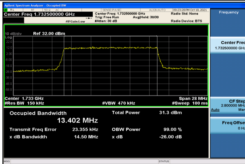
Band4-15MHz-16QAM-20175-75RB#0-13.402
