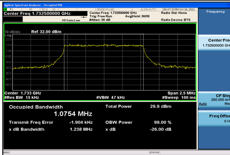
Band4-1.4MHz-16QAM-20175-6RB#0-1.0754
