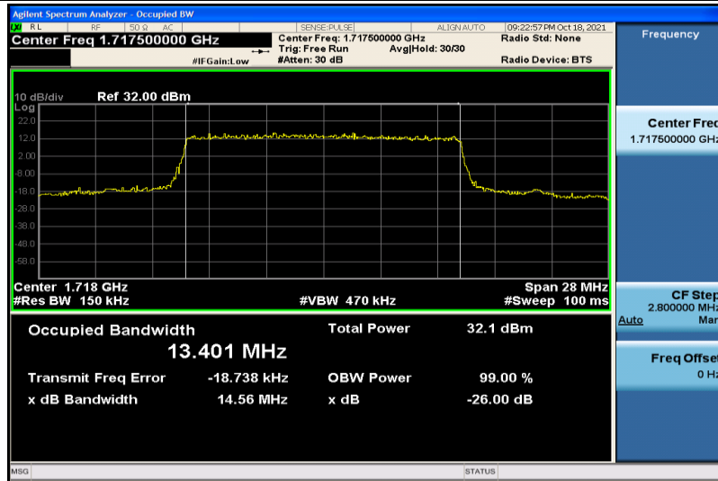
Band4-15MHz-QPSK-20025-75RB#0-13.401
