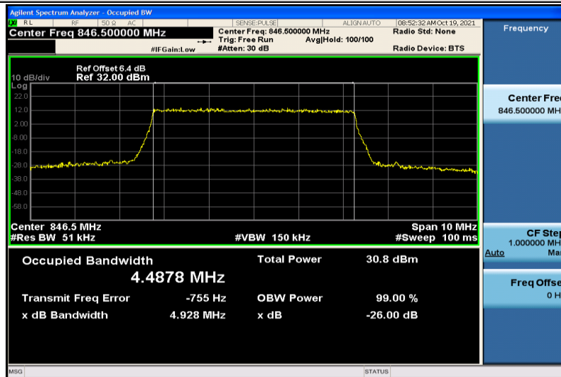
Band5-5MHz-QPSK-20625-25RB#0-4.4878
