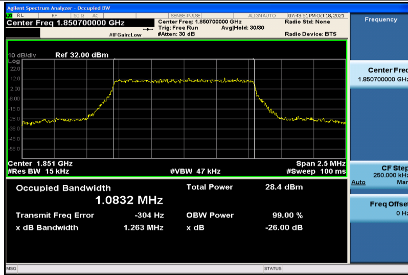
Band2-1.4MHz-16QAM-18607-6RB#0-1.0832
