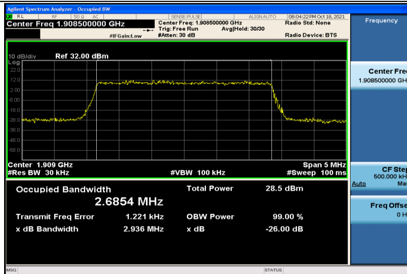
Band2-3MHz-16QAM-19185-15RB#0-2.6854
