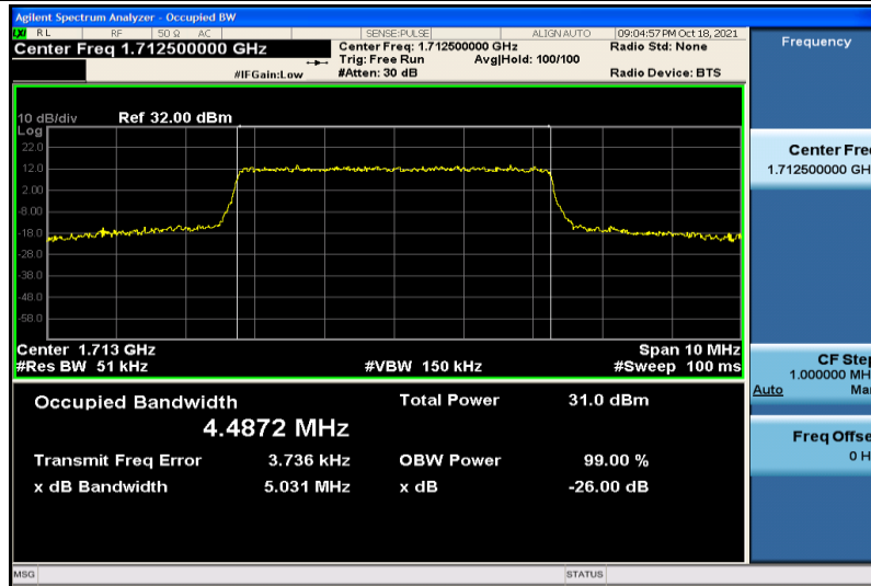
Band4-5MHz-16QAM-19975-25RB#0-4.4872
