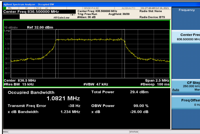
Band5-1.4MHz-QPSK-20525-6RB#0-1.0821
