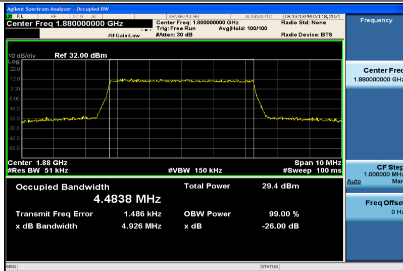
Band2-5MHz-16QAM-18900-25RB#0-4.4838
