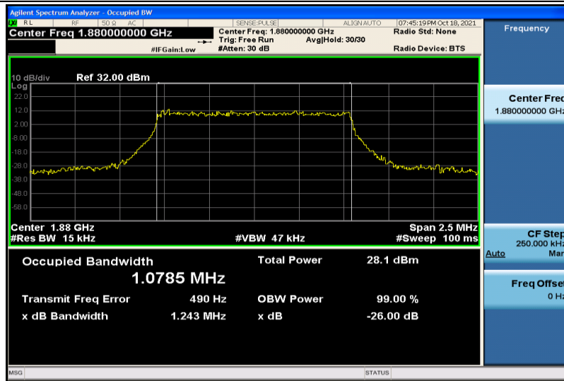
Band2-1.4MHz-16QAM-18900-6RB#0-1.0785
