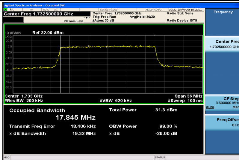
Band4-20MHz-16QAM-20175-100RB#0-17.845
