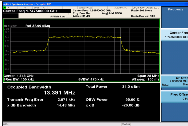
Band4-15MHz-QPSK-20325-75RB#0-13.391
