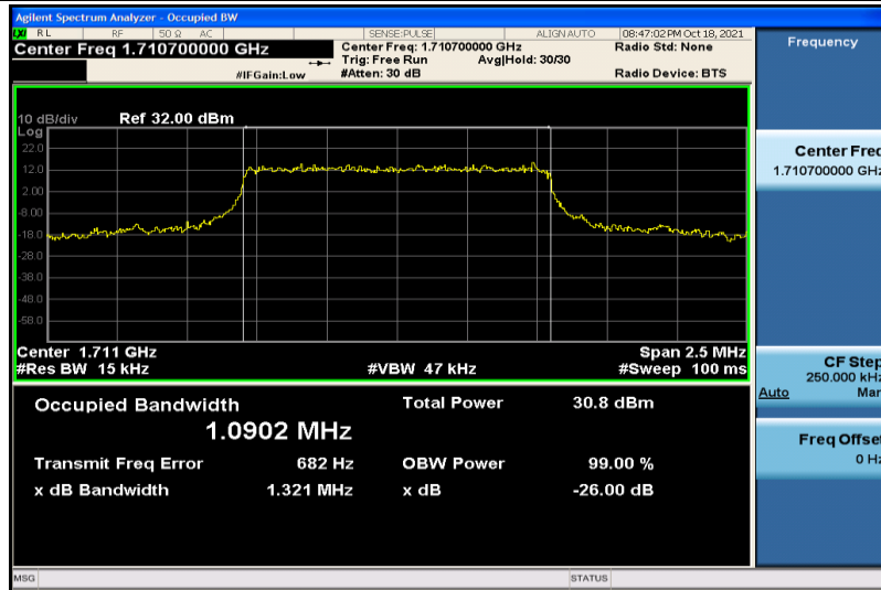
Band4-1.4MHz-QPSK-19957-6RB#0-1.0902
