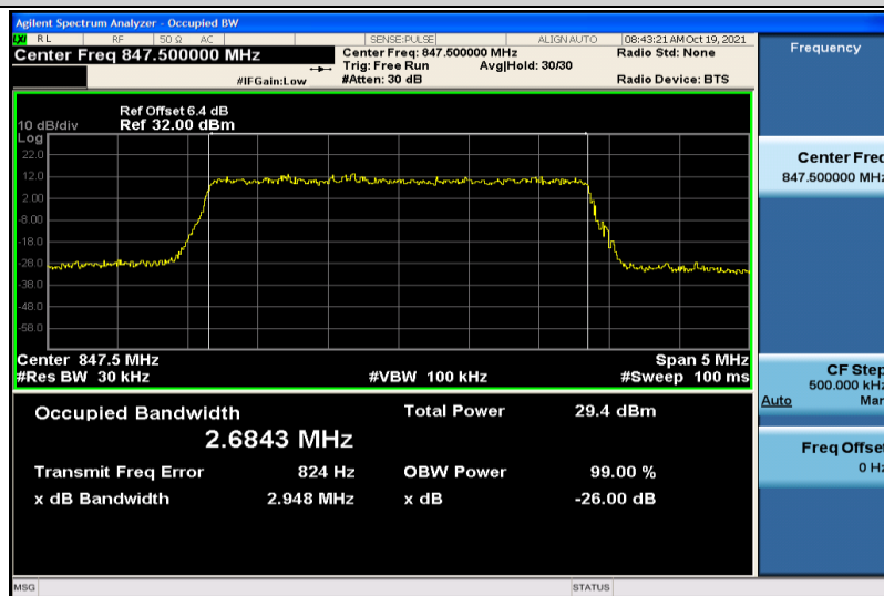
Band5-3MHz-16QAM-20635-15RB#0-2.6843
