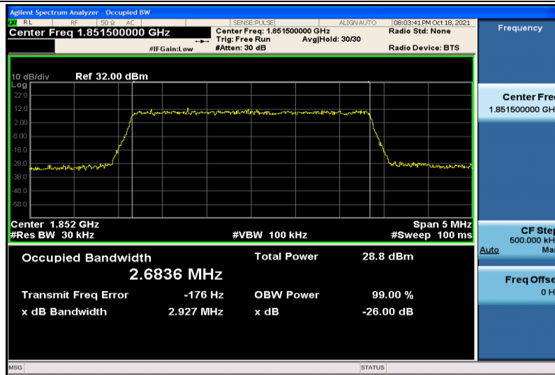
Band2-3MHz-16QAM-18615-15RB#0-2.6836
