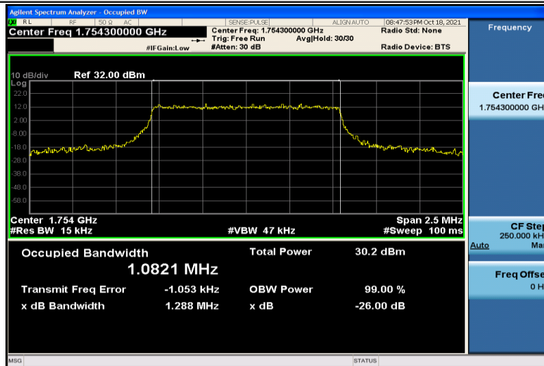
Band4-1.4MHz-16QAM-20393-6RB#0-1.0821
