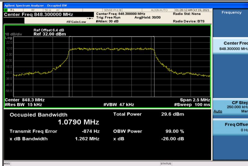
Band5-1.4MHz-QPSK-20643-6RB#0-1.0790
