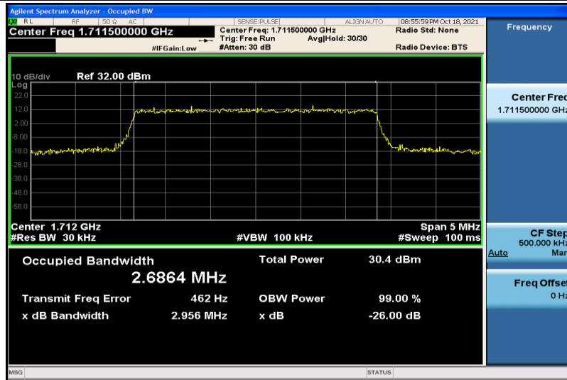
Band4-3MHz-16QAM-19965-15RB#0-2.6864
