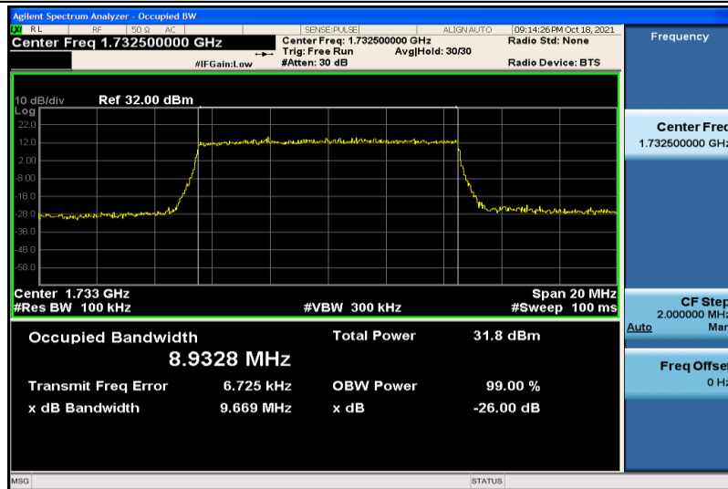
Band4-10MHz-QPSK-20175-50RB#0-8.9328
