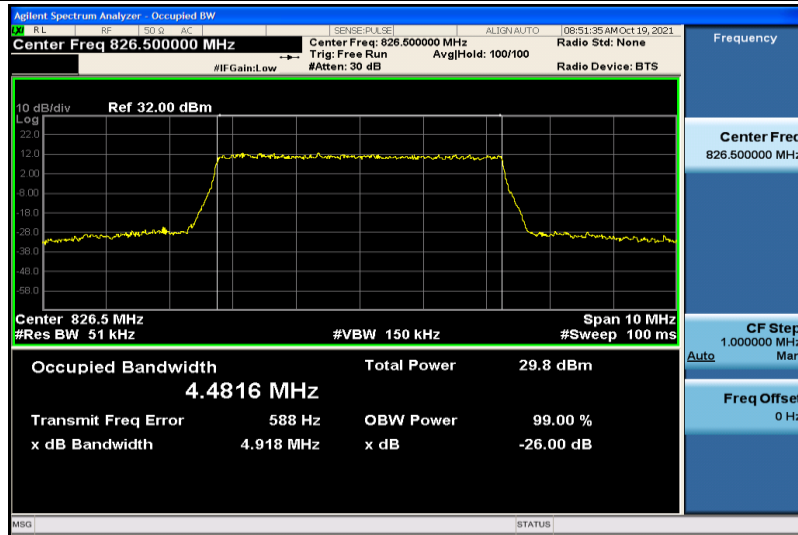
Band5-5MHz-16QAM-20425-25RB#0-4.4816
