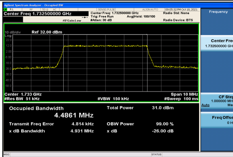
Band4-5MHz-16QAM-20175-25RB#0-4.4861
