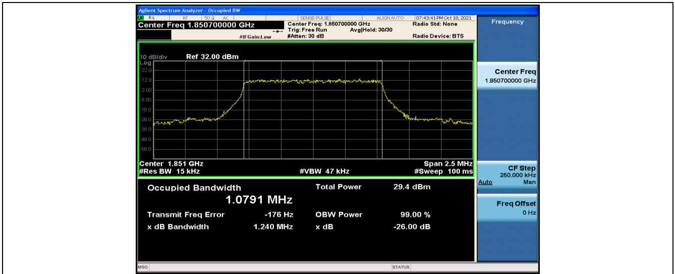
Band2-1.4MHz-QPSK-18607-6RB#0-1.0791
