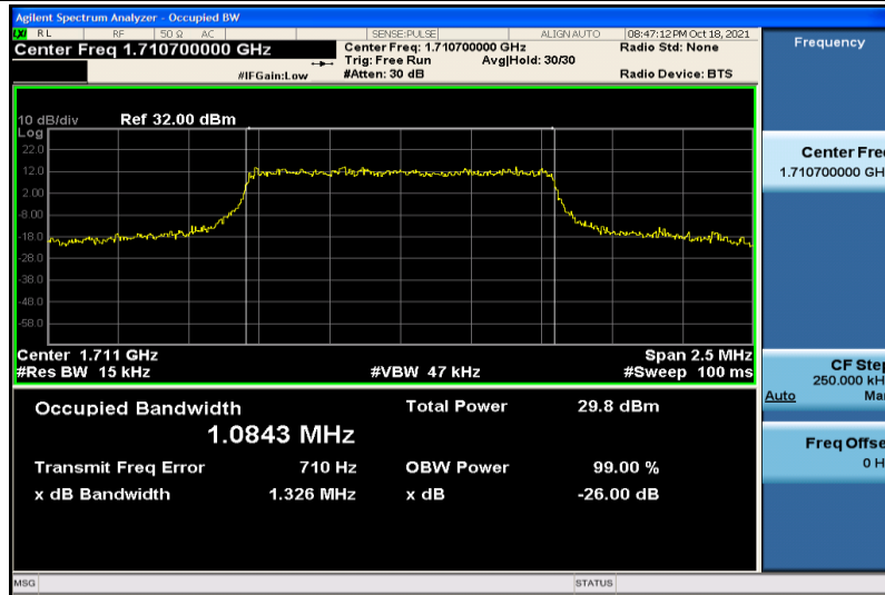
Band4-1.4MHz-16QAM-19957-6RB#0-1.0843
