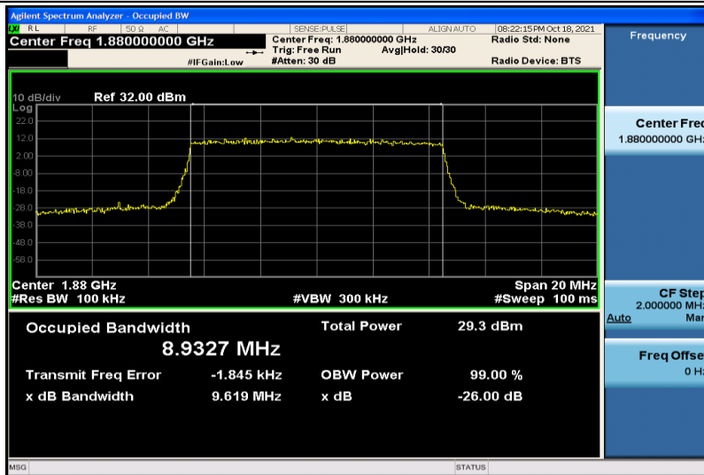
Band2-10MHz-16QAM-18900-50RB#0-8.9327
