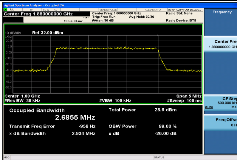
Band2-3MHz-16QAM-18900-15RB#0-2.6855
