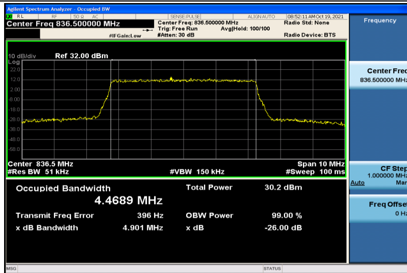
Band5-5MHz-16QAM-20525-25RB#0-4.4689
