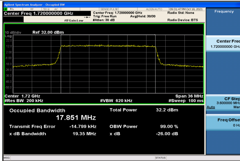
Band4-20MHz-QPSK-20050-100RB#0-17.851
