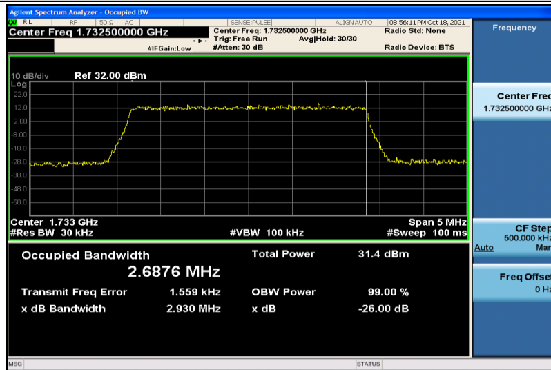
Band4-3MHz-QPSK-20175-15RB#0-2.6876
