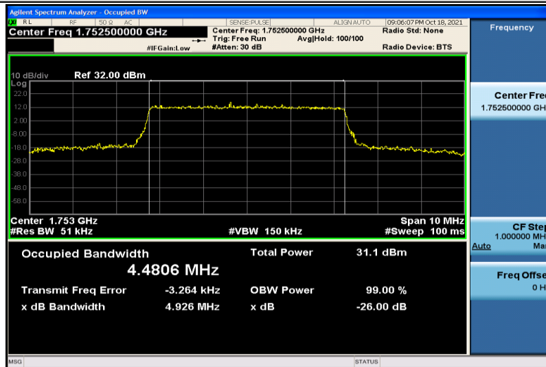
Band4-5MHz-16QAM-20375-25RB#0-4.4806
