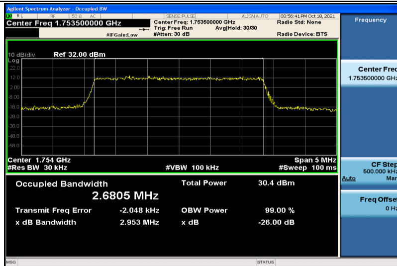
Band4-3MHz-16QAM-20385-15RB#0-2.6805
