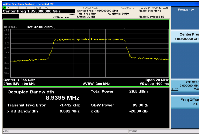
Band2-10MHz-16QAM-18650-50RB#0-8.9395
