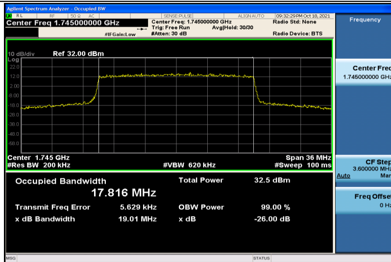
Band4-20MHz-QPSK-20300-100RB#0-17.816
