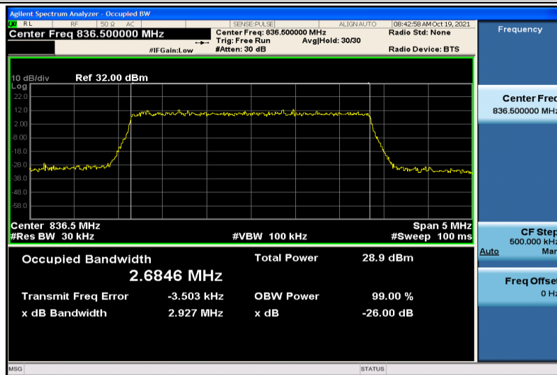
Band5-3MHz-16QAM-20525-15RB#0-2.6846
