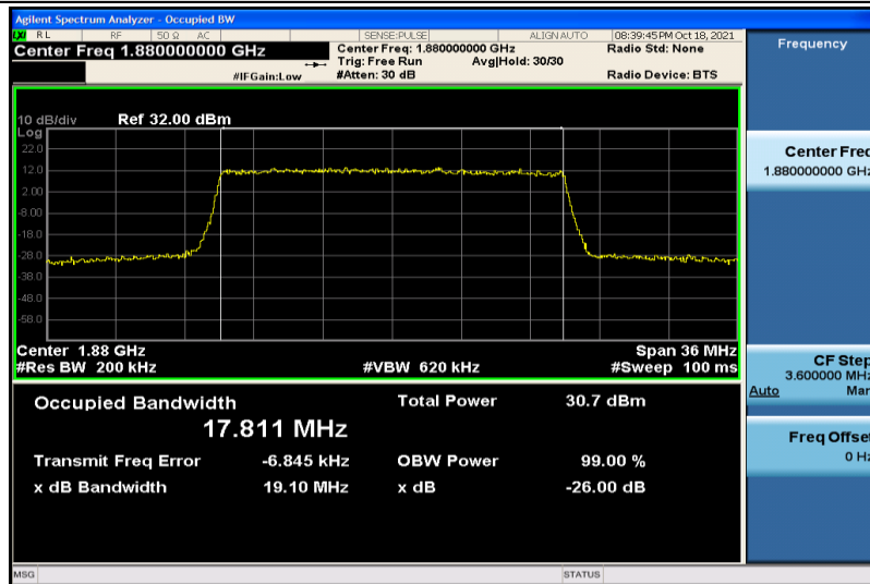
Band2-20MHz-QPSK-18900-100RB#0-17.811
