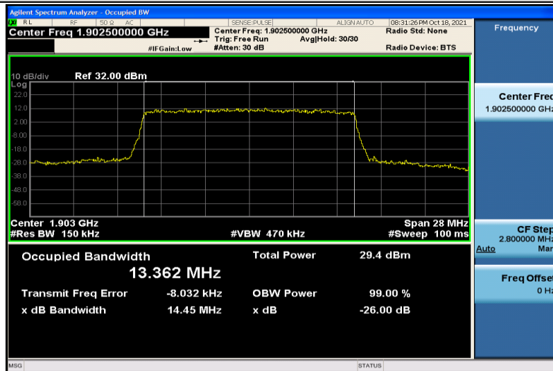
Band2-15MHz-16QAM-19125-75RB#0-13.362
