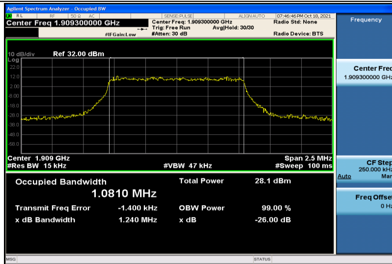
Band2-1.4MHz-16QAM-19193-6RB#0-1.0810
