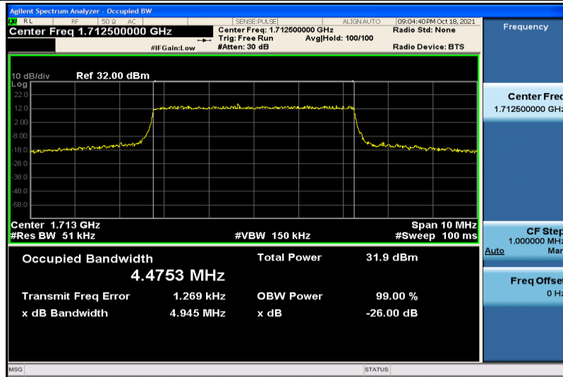
Band4-5MHz-QPSK-19975-25RB#0-4.4753
