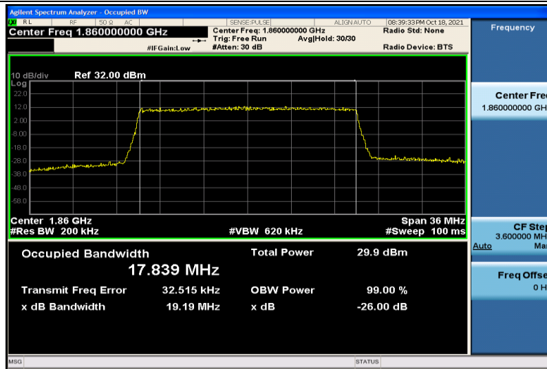
Band2-20MHz-16QAM-18700-100RB#0-17.839
