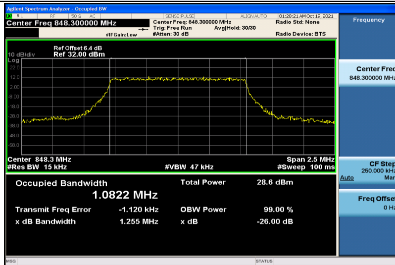
Band5-1.4MHz-16QAM-20643-6RB#0-1.0822
