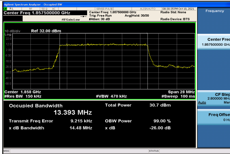
Band2-15MHz-QPSK-18675-75RB#0-13.393
