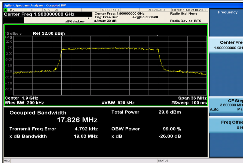
Band2-20MHz-16QAM-19100-100RB#0-17.826
