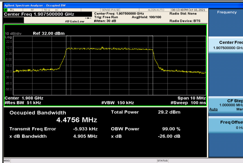
Band2-5MHz-16QAM-19175-25RB#0-4.4756
