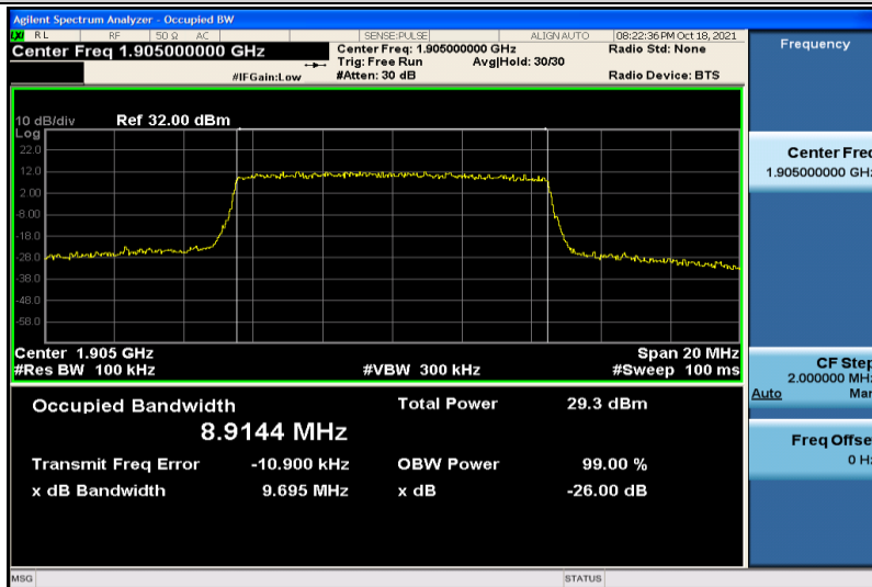
Band2-10MHz-16QAM-19150-50RB#0-8.9144
