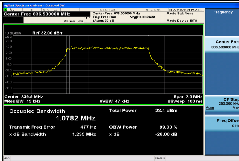
Band5-1.4MHz-16QAM-20525-6RB#0-1.0782
