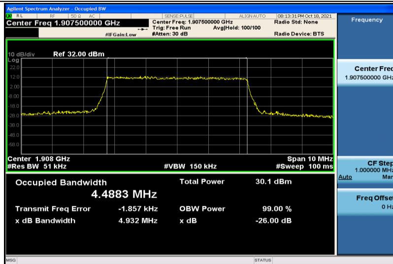
Band2-5MHz-QPSK-19175-25RB#0-4.4883
