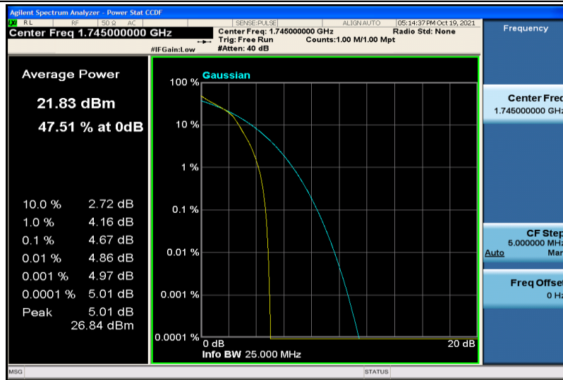
Band66-3MHz-16QAM-132322-15RB#0
