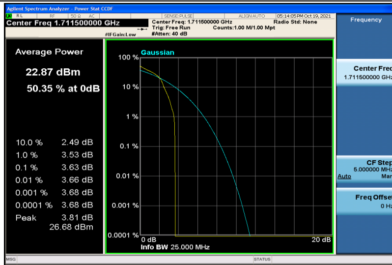
Band66-3MHz-16QAM-131987-1RB#0
