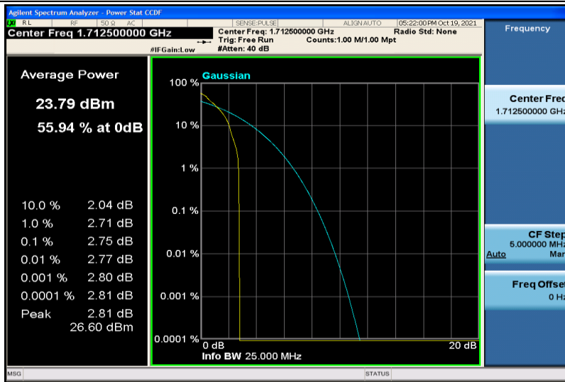
Band66-5MHz-QPSK-131997-1RB#0
