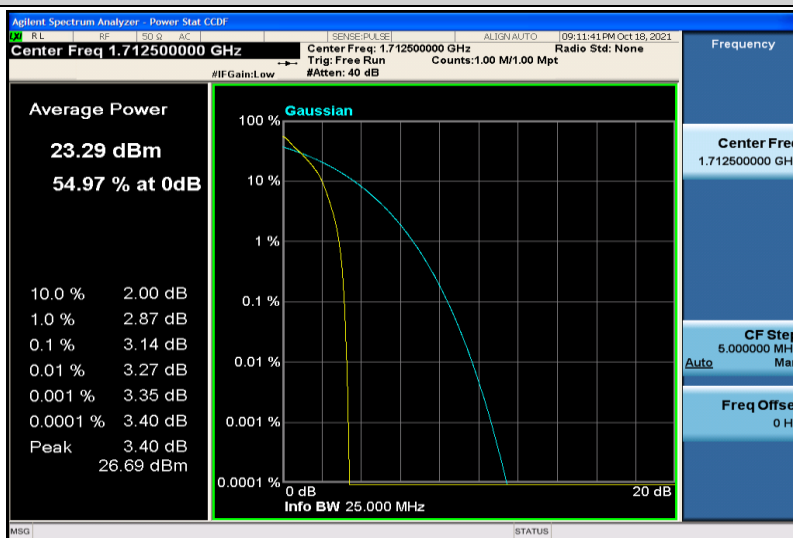
Band4-5MHz-QPSK-19975-25RB#0
