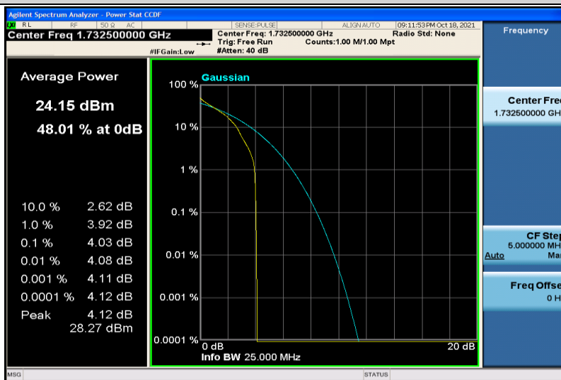
Band4-5MHz-QPSK-20175-1RB#0
