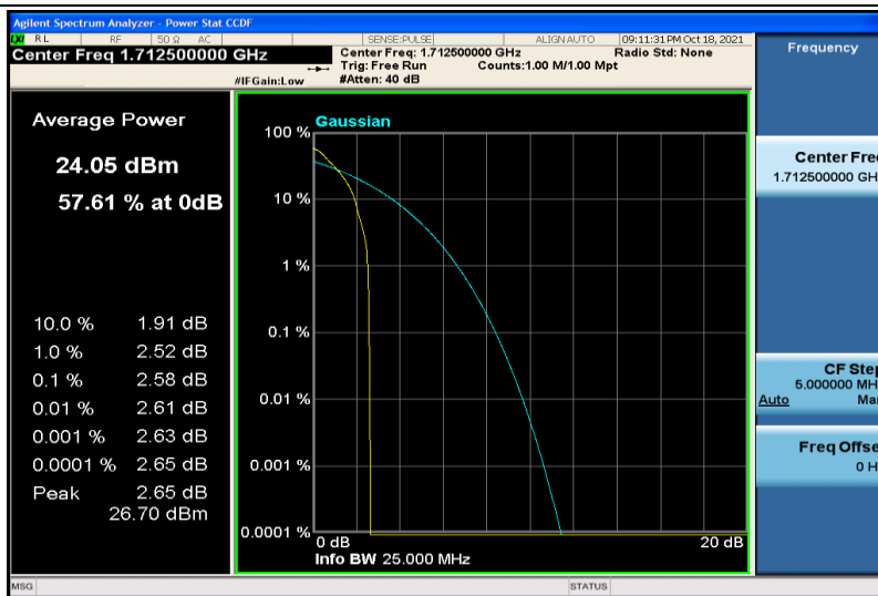
Band4-5MHz-QPSK-19975-1RB#0
