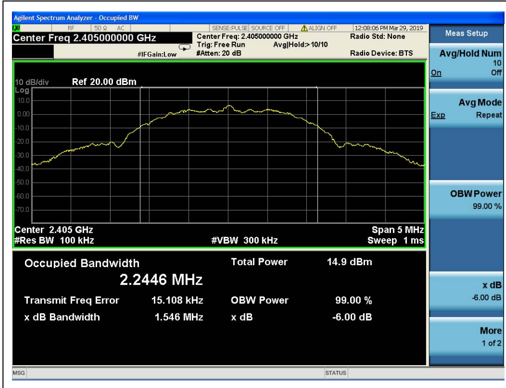
(Channel 11, 2405MHz)
