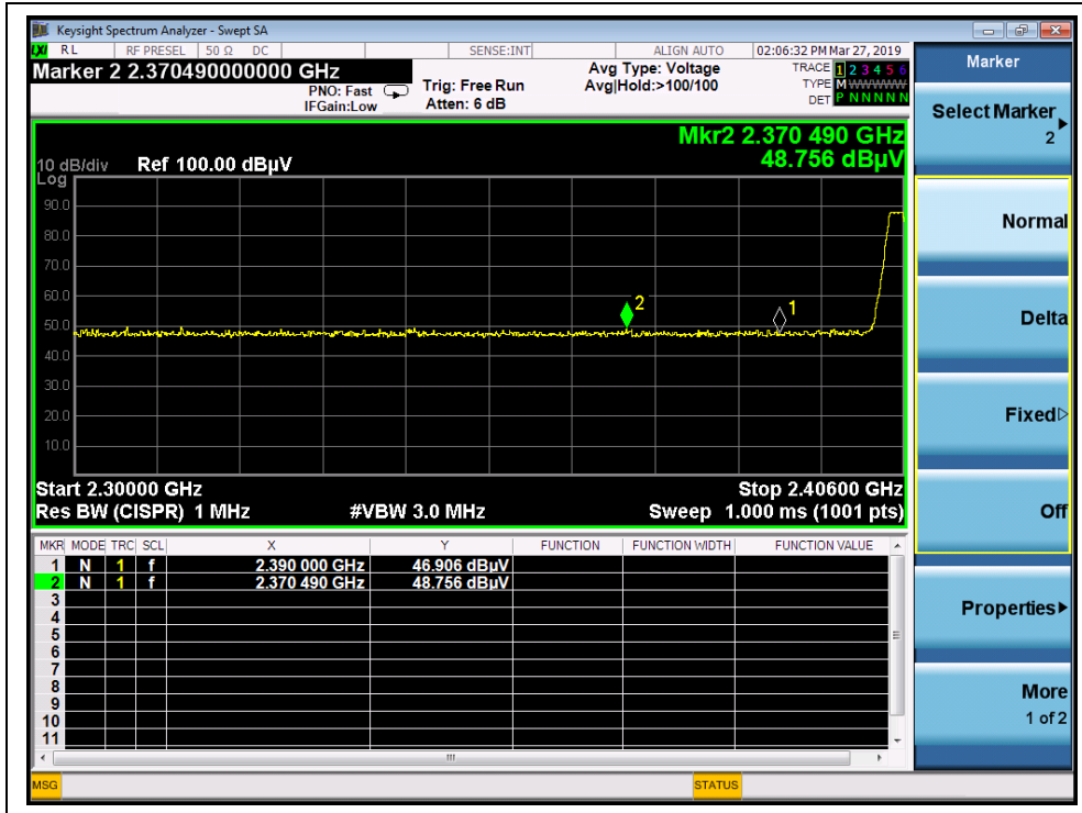
(Channel = 11, PEAK)
