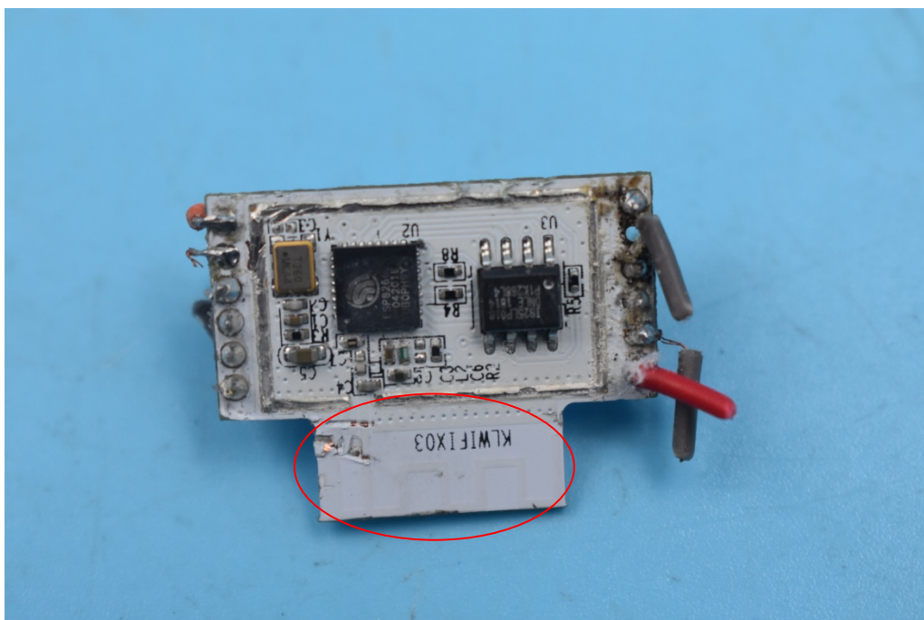
4. WIFI antenna view
