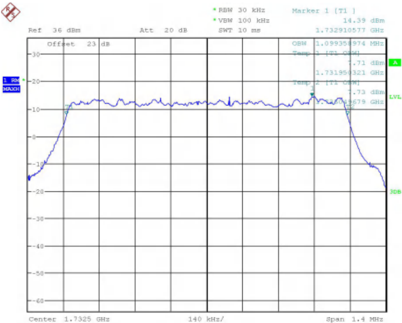
Band4-99% OBW-1.4MHz Bandwidth-16QAM
