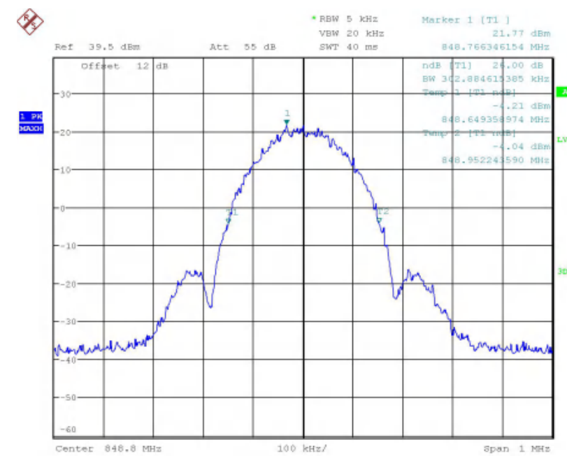
99% OBW-8PSK-Channel 251
