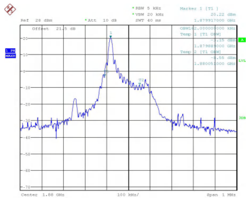
Band2-99% OBW-Middle Channel-BPSK
