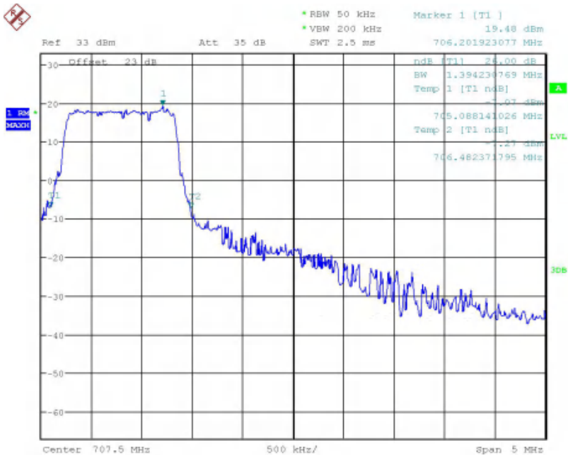
Band12-26dB OBW-5MHz Bandwidth-16QAM
