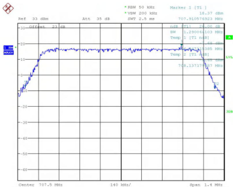
Band12-26dB OBW-1.4MHz Bandwidth-16QAM
