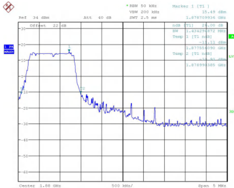
Band2-26dB OBW-5MHz Bandwidth-16QAM
