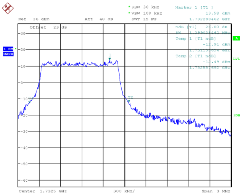
Band4-26dB OBW-3MHz Bandwidth-16QAM
