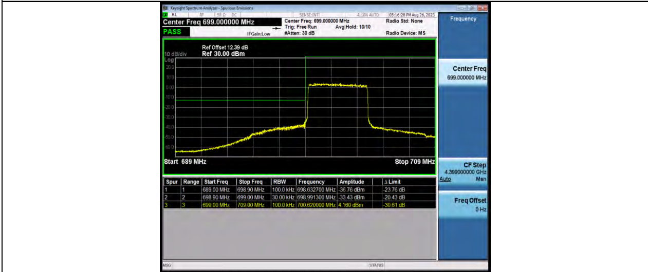
Band12-5MHz-16QAM-23155-1RB#24
