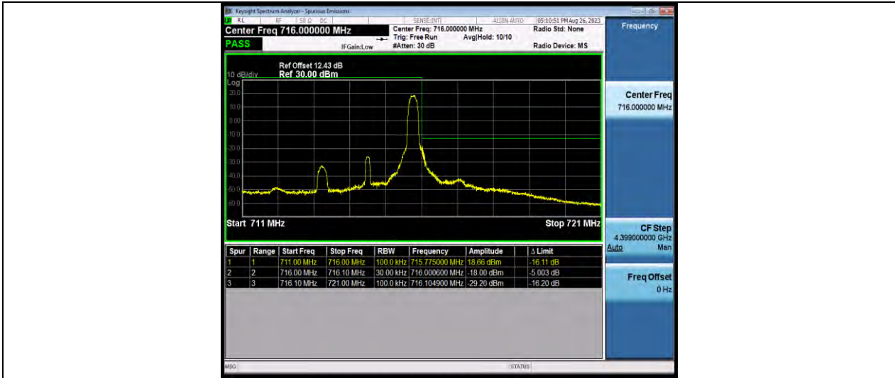
Band12-3MHz-16QAM-23165-15RB#0
