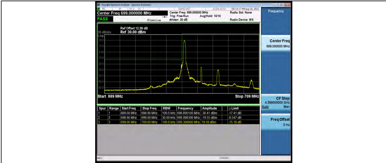
Band12-5MHz-16QAM-23035-25RB#0
