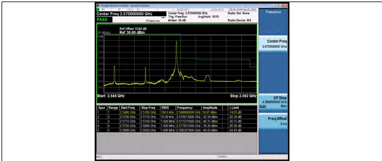
Band7-20MHz-QPSK-21350-100RB#0
