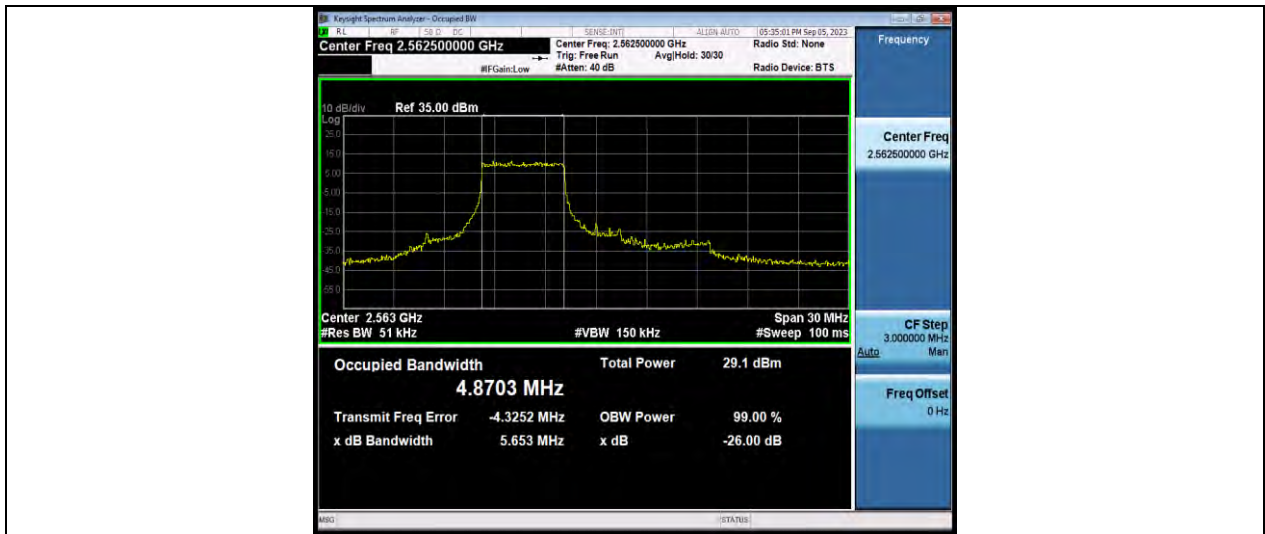
Band7-20MHz-QPSK-20850-100RB#0
