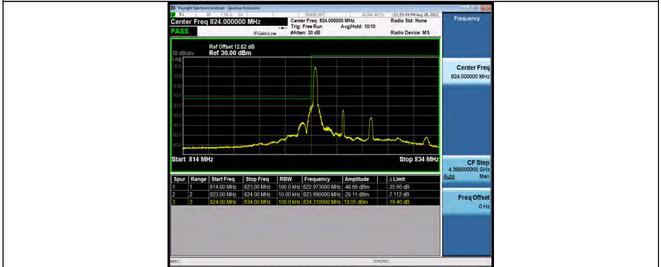
Band26-5MHz-QPSK-26815-25RB#0
