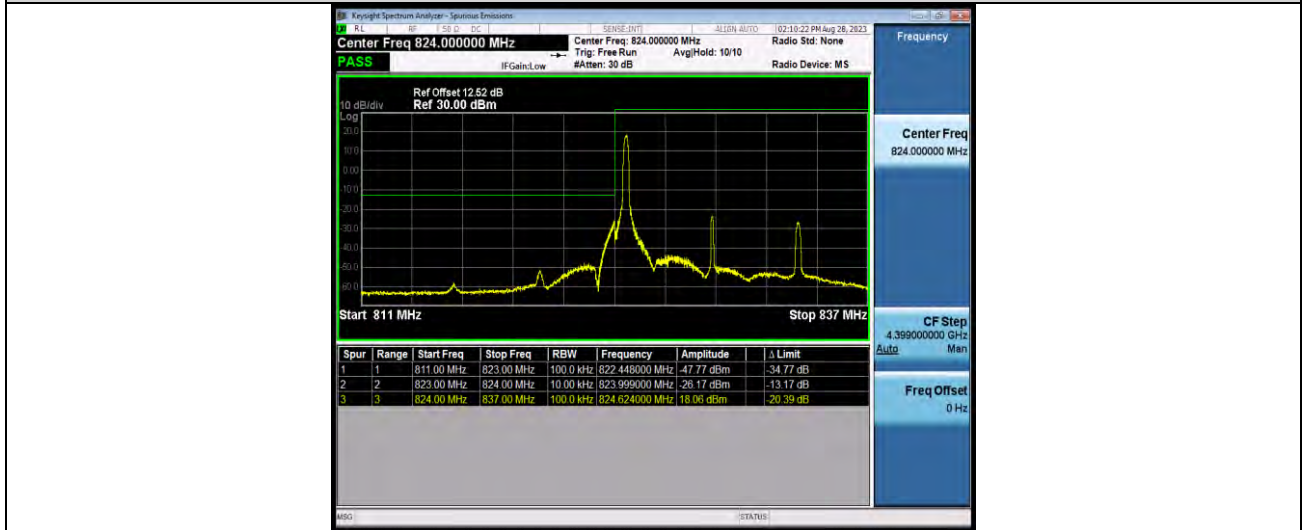
Band26-10MHz-16QAM-26840-27RB#0
