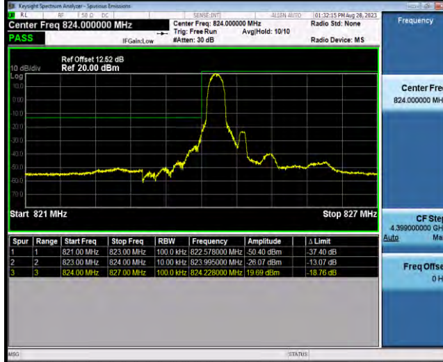
Band26-1.4MHz-QPSK-26797-6RB#0
