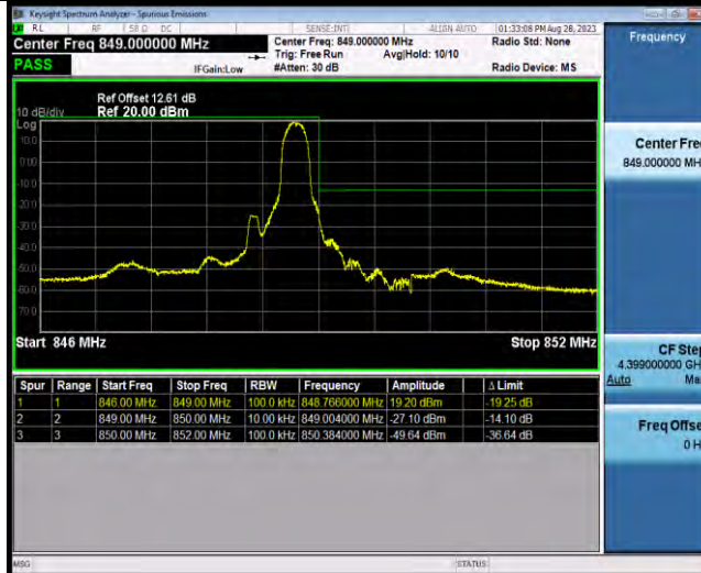
Band26-1.4MHz-QPSK-27033-1RB#5
