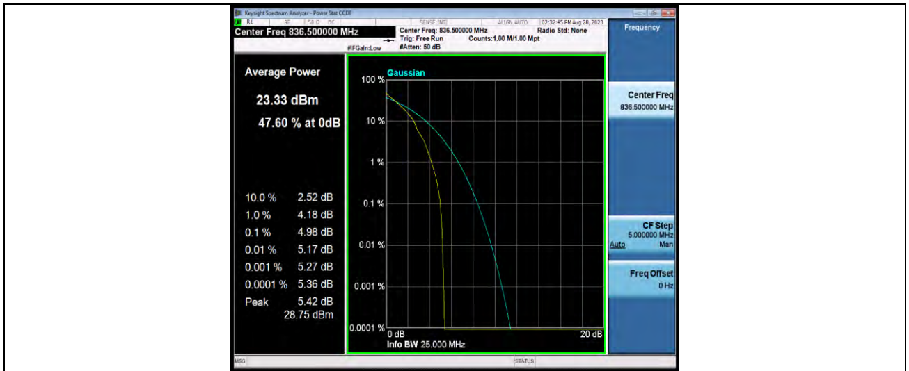
Band26-15MHz-QPSK-26915-75RB#0
