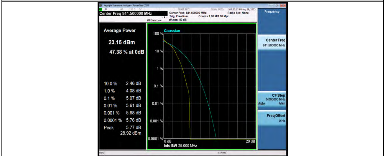
Band26-15MHz-QPSK-26965-75RB#0
