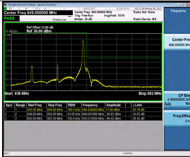
Band26-10MHz-16QAM-26990-27RB#23
