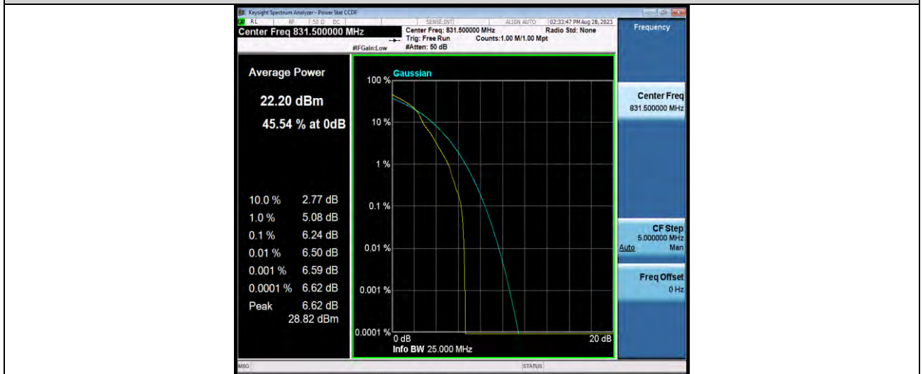
Band26-15MHz-16QAM-26865-27RB#0
