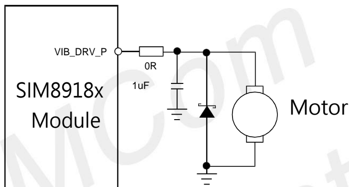
Figure 33: Motor Interface Reference Design
