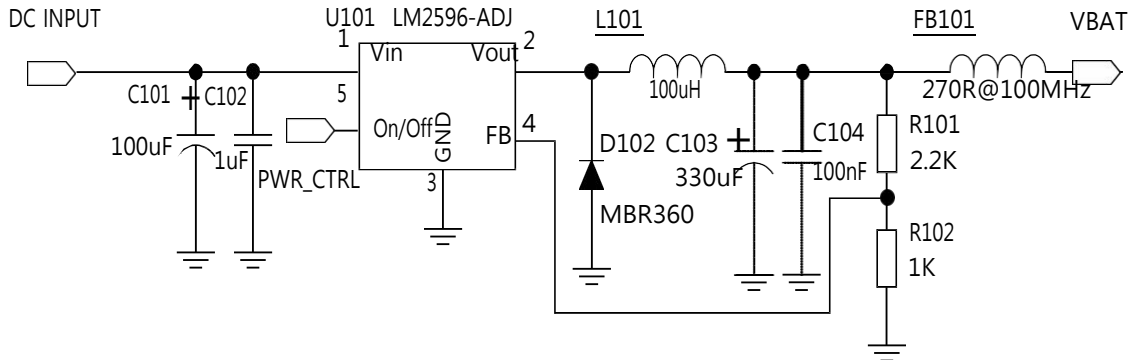
Figure 6: DC-DC Power Supply Reference Design
