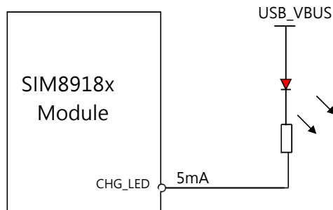
Figure 34: LEDs Interface Reference Design
