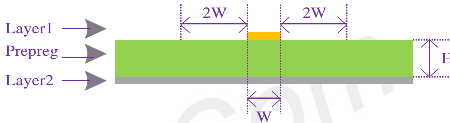
Figure 42: Two Layers PCB Microstrip-slot Line Structure
